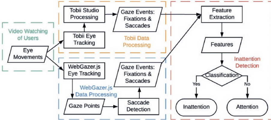
Figure 4.2: Overview of the processing pipeline
