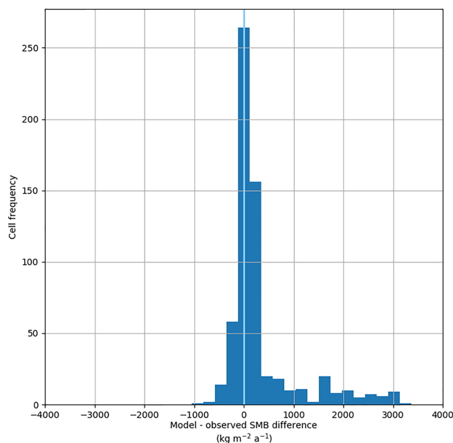
Figure 12. Histogram of differences between modeled and observed annual SMB, at all collected pit/core locations as detailed in Sect. 2 from ablation and accumulation zones. The light blue line highlights 0 difference between model and observed; values above (below) this line indicate that the model overestimates (underestimates) SMB in comparison to the observations.
