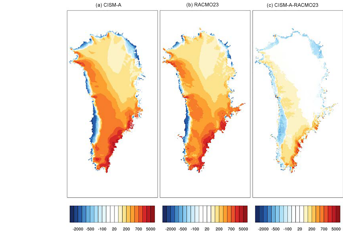
Figure 2. Surface mass balance contours for (a) CISM-A forced with RACMO2.0, (b) RACMO2.3, and (c) CISM-A minus RACMO2.3, with CISM-A interpolated to the coarser RACMO2.3 grid.
