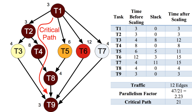
FIGURE 1. A task graph, with task timing and dependencies.
