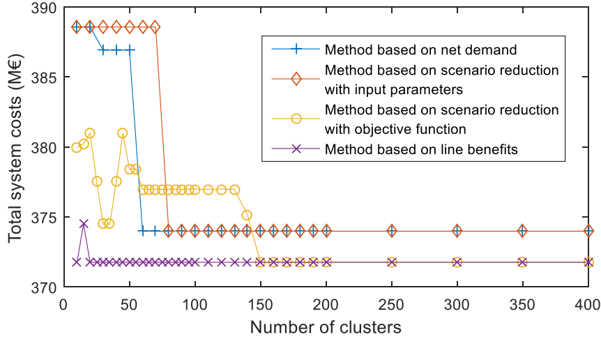
Fig. 4.6. Case B: Evolution of total system costs with the number of snapshots considered when these are selected 1) with the method proposed here, 2) according to the net demand in the system nodes (1 st alternative approach), 3) with the scenario reduction technique based on total system costs (2 nd alternative approach), and 4) with the scenario reduction technique based on input parameters (3 rd alternative approach).
