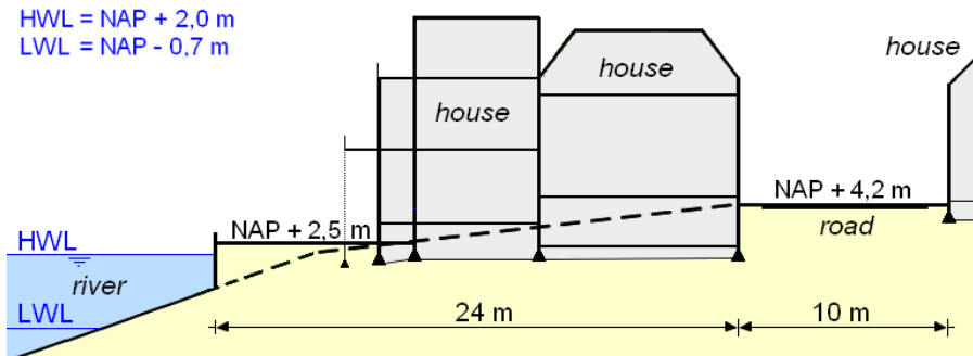
Figure 6.39: Slidrecht, cross-section AA of the dike at the considered project location. HWL = high water level; LWL = low water level)
