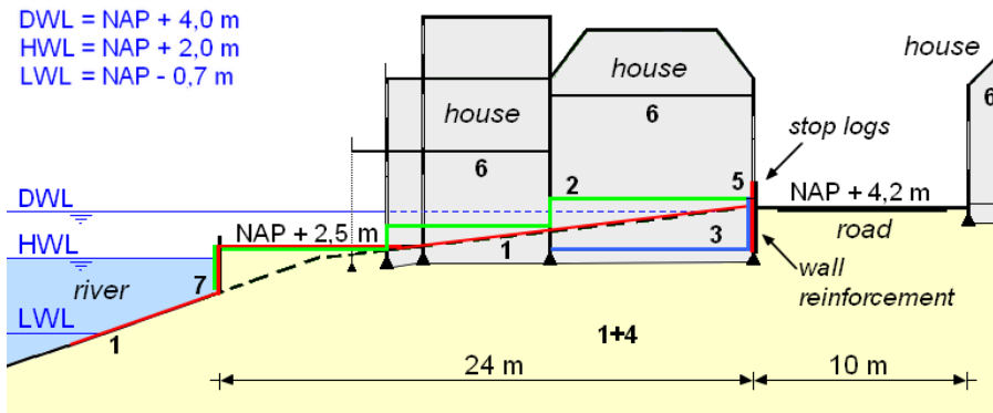
Figure 6.41: Sliedrecht river dike: Design concept 2: 'Water-retaining inner façade'
