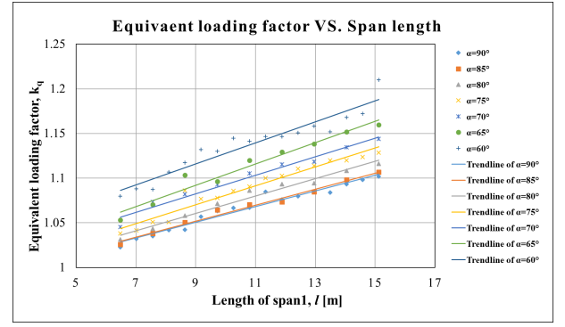
Figure 18: Equivalent loading factor versus span length
