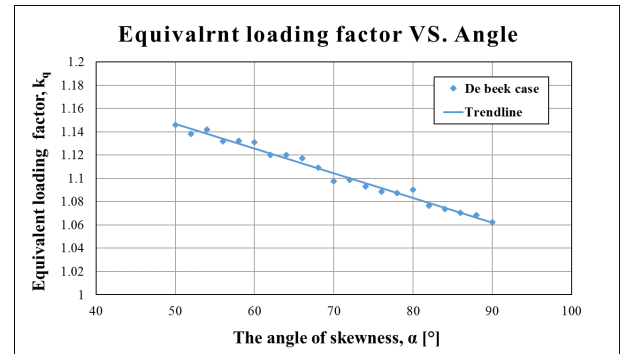
Figure 14: Equivalent loading factor versus skewness
