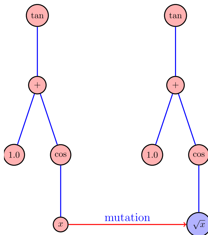
Fig. 12. Example of mutation process for the mathematical function \tan(1 + \cos(x)) .
