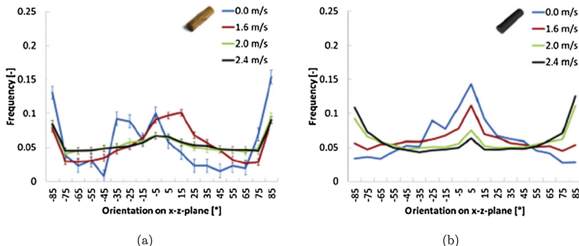
Fig. 23. Distribution of the orientation of elongated cylinders (4 mm × 14 mm) along the x-z plane from (a) CFD-DEM simulations and (b) experiments. Best correspondence between simulations and experiments occurs at high gasification velocities when particles align with the direction of flow. Images from Vollmari et al. (2016).
