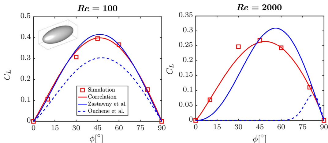
Fig. 8. Comparison of C_L using various correlation functions for a prolate spheroid for varying incident angle and Re . Images based on those in Sanjeevi et al. (2018).
