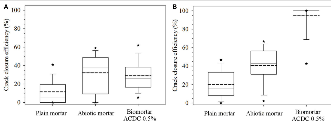
FIGURE 2 | Data depicting crack closure performances of different series obtained for the first 14 days (A) and at the end of 28 days (B) . Each box plot represents the crack closure performance data for 60 data points collected along the cracks of 10 separate specimens. The dashed line represents the mean crack closure percentage; the top, middle and bottom lines are the 75, 50, and 25th percentiles, respectively. The whiskers shows the minimum and maximum crack closure. *Indicates 5th/95th percentiles.
