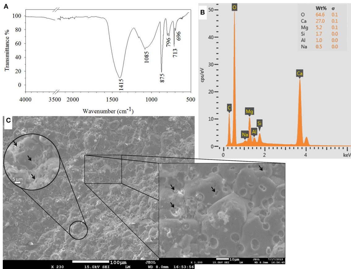
FIGURE 7 | Characterization of the healing material as calcium carbonate in FTIR spectrum of the scraped material from the inner crack surface (A); in EDS analysis (B); and in SEM micrographs of the inner crack surface of the healed biomortar (C). Arrows indicate either clusters of bacteria or traces of a single bacterium on precipitated calcium carbonate.
