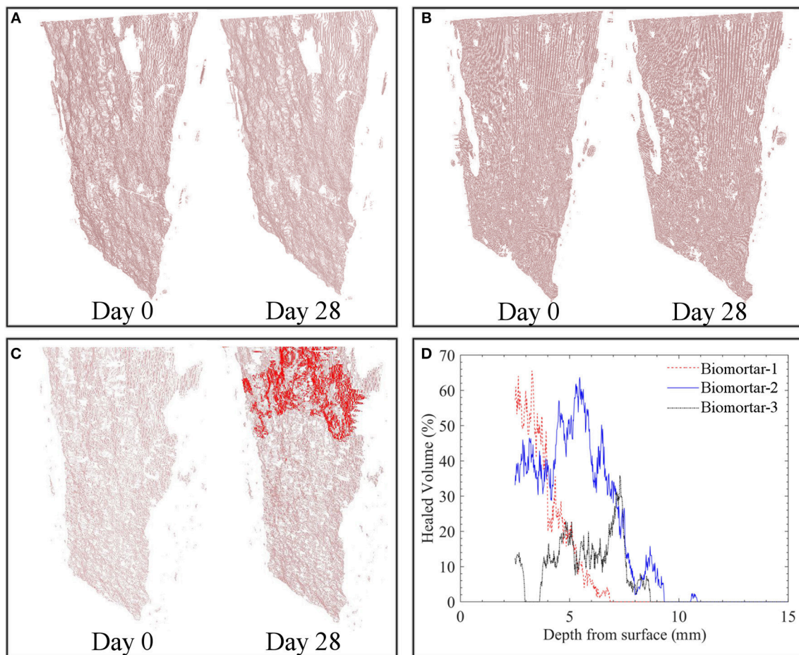
FIGURE 5 | Spatial distribution of the calcium carbonate inside the extracted crack volume before and after 28 days tap water treatment of plain control specimens (A); abiotic control specimens (B); biomortars (C) and the crack closure percentage at 16.6 μm layered increments starting from the surface (D). Red zones represent MICP and pinkish zones represent the empty crack. For interpretation of the references to color in this figure legend, the reader is referred to the web version of this article.
