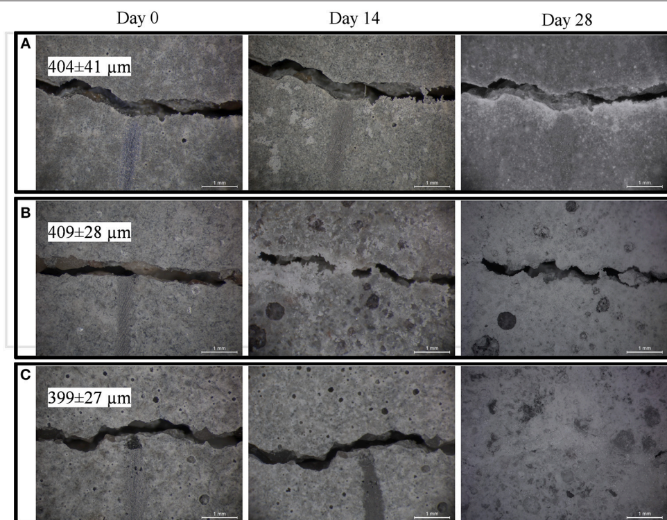
FIGURE 3 | Micrographs showing biweekly evolution of the crack at the specimen surface in plain control series (A) ; abiotic control series (B) ; biomortars containing ACDC biogranules (C) . Crack widths are given as mean \pm standard deviation ( n = 10 ).
