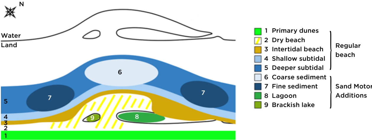
Figure 3. Bird's eye view illustration of the ecological zones created by the Sand Motor.
