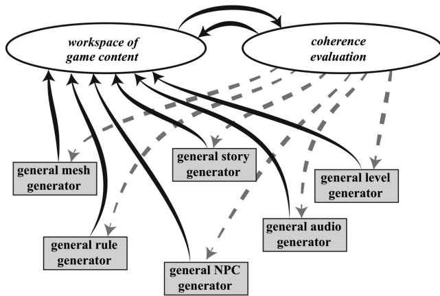
Fig. 5. Example bottom-up generative approach based on an external or internal system that evaluates the components' consistency and playability as a whole and may adapt the individual generators' parameters (shown as dashed arrows) based on these evaluations.
