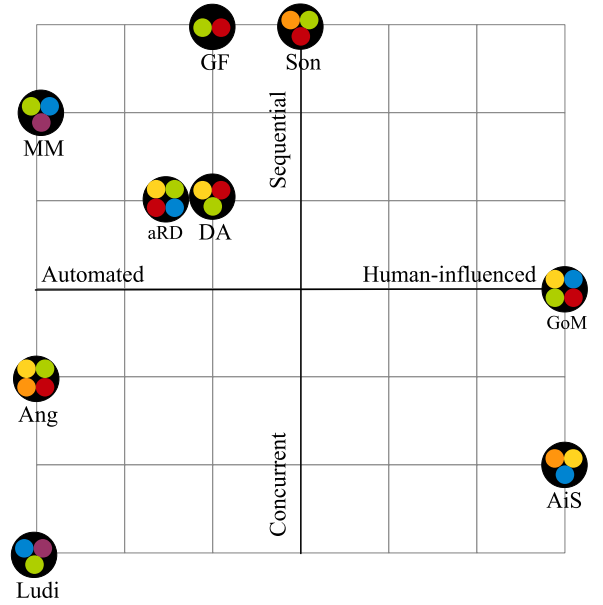
Fig. 16. Spectrum of the case studies on orchestration.
