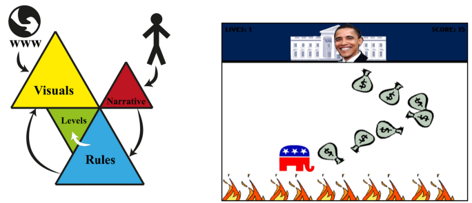
Fig. 8. Facet orchestration in Game-O-Matic, where a human-authored microrhetoric (small-scale narrative) informs which game objects and rules exist in the gameworld; game objects get their visuals from online sources through a search query based on the microrhetoric. In-game screenshot is from [89].
