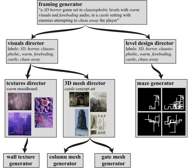
Fig. 4. Example top-down generative process based on frames that are refined by subsequent generators (as directors ).
