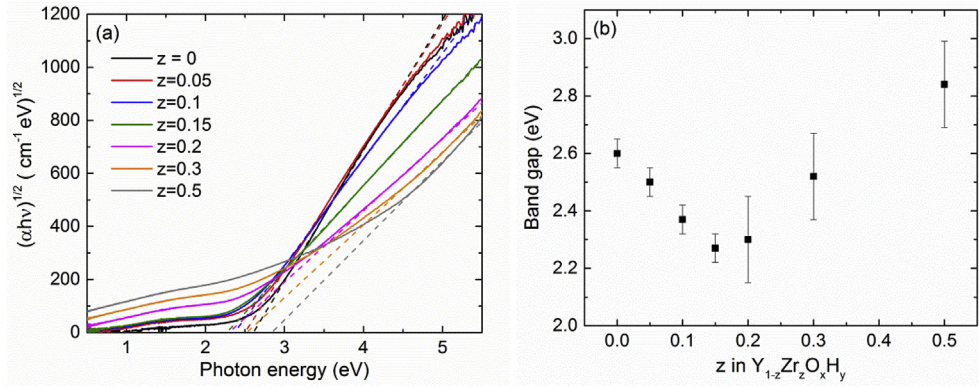
Fig. 4. (a) Tauc plots of Y_{1-x}Zr_xO_xH_y films for different Zr fractions. An absorption tail at lower photon energies is observed and increases to higher absorption values as Zr is added to the system. (b) Optical band gap of Y_{1-x}Zr_xO_xH_y versus the Zr fraction.
