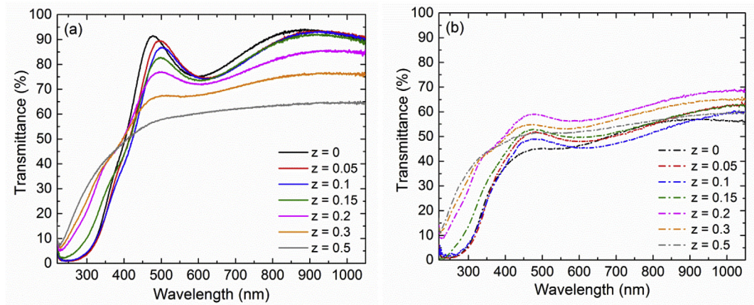
Fig. 5. Spectral transmittance of Y_{1-x}Zr_xO_xH_y films ( d \approx 230 nm): (a) before illumination and (b) after UV illumination.
