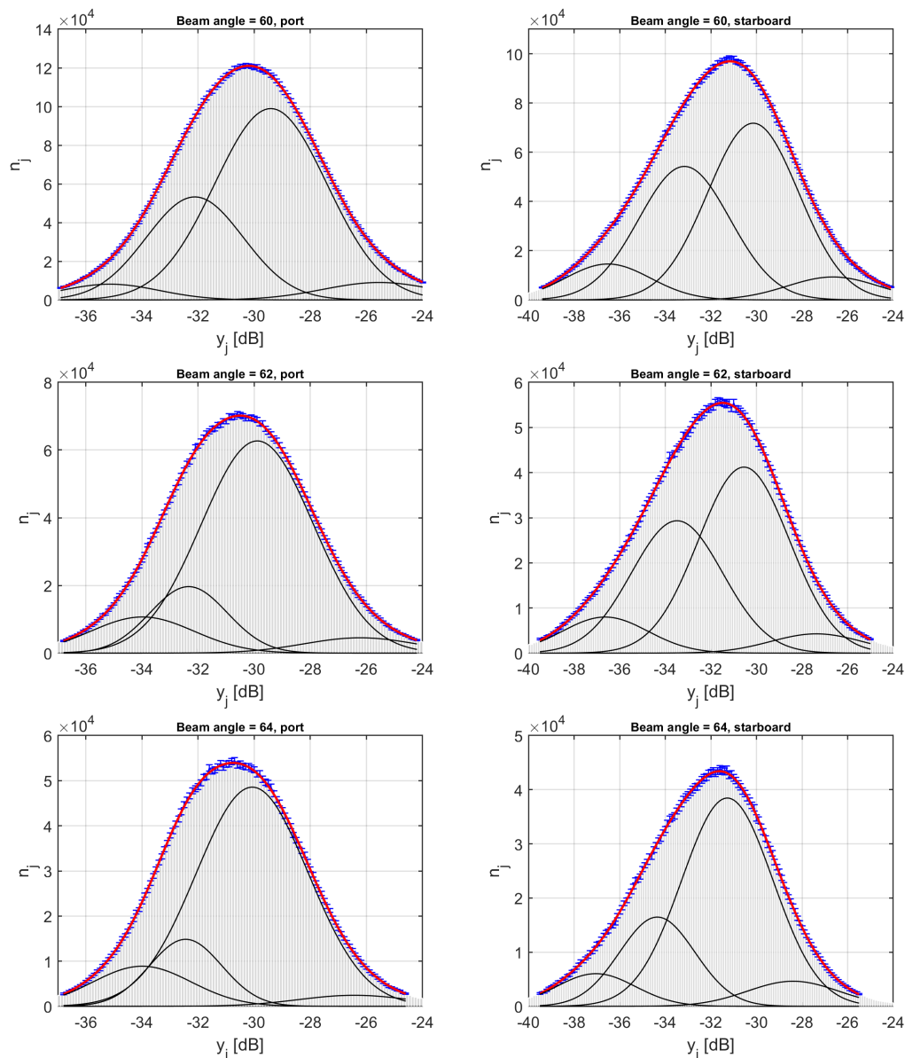
Figure 6. Measured histograms for grazing angles 30^\circ , 28^\circ , and 26^\circ for both port and starboard sides, in gray; sum of m = 4 number of Gaussians, in red (see: Equation (4)), individual Gaussians are in black. Error bars (in blue) were multiplied by a factor of 3 for distinction.
