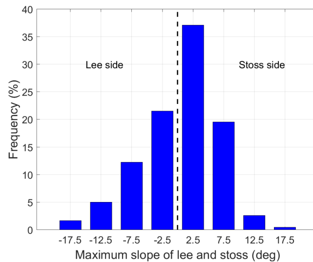
Figure 17. Histogram of maximum slopes computed in 32 typical areas with megaripple structures.
