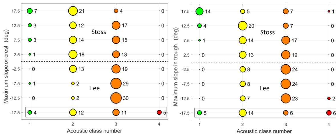
Figure 18. Acoustic classification results of 32 typical areas with megaripple structure given for bin centers ranging from -17.5 to 17.5 degrees; crest (left), trough (right).
