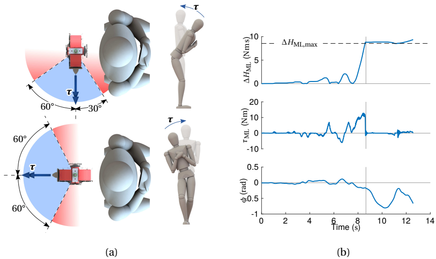
Supplementary Fig. 4.A2: Geometric saturations. (a): Overhead views showing the ranges of gimbal operation (in blue) for AP (top) and ML (bottom) torque ( \tau ) generation. When the gimbal rotates such that \tau approaches the boundary, the gimbal is arrested and torque generation ceases, referred to here as geometric saturation of the gyroscopic actuator. (b): Example timeseries data of subject C14 of Experiment 1, showing the occurrence of geometric saturation (vertical line) with the ‘spring’ (S) controller. As the subject leans ( \phi ), the controller produces an opposing torque ( \tau ); the gimbal reaches its limit when the time integral of the torque (the exchanged angular momentum in this direction, \Delta H_{ML} ) reaches a maximum ( \Delta H_{ML,max} ), at which point \tau ceases.
