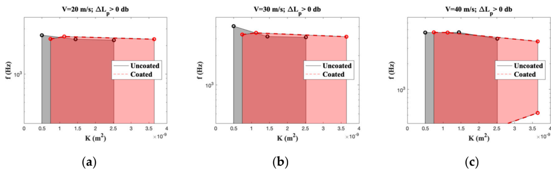
Figure 9. Comparison of frequency range f for which noise reduction is positive at different permeabilities K for different free-stream air velocities: (a) v = 20 m/s, (b) v = 30 m/s, and (c) v = 40 m/s.
