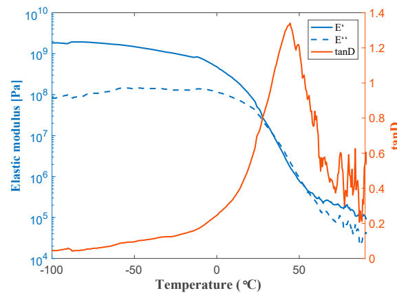
Figure 5. DMA measurements for solvent-based paint system.
