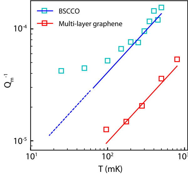
Figure 5. Temperature-dependent energy dissipation ( Q_m^{-1} ) of BSCCO mechanical resonator (cyan-squares). The measurements were performed at cavity injected power of -83 dBm and at V_{dc} = 0.6 V. For comparison, similar results from a multilayer graphene resonator are plotted (red-squares). Blue and red solid lines are guides plotted with a temperature exponent of 0.75.
