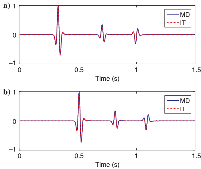
Figure 6. (a) A comparison of zero-offset traces from the modeled primary reflections (MD) and retrieved data sets (IT) and (b) a comparison of the nonzero-offset (1000 m) traces.
