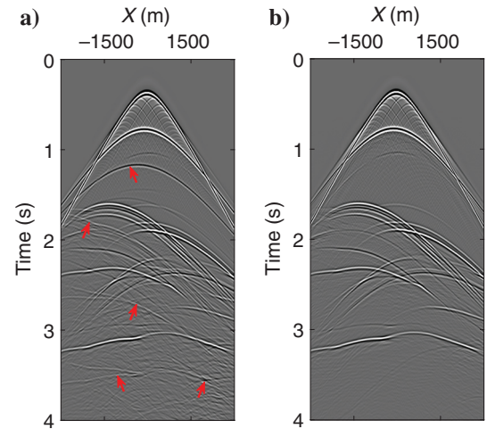
Figure 8. (a) The modeled reflection response and (b) the retrieved primary reflections using equation 21. The red arrows indicate internal multiple reflections.
