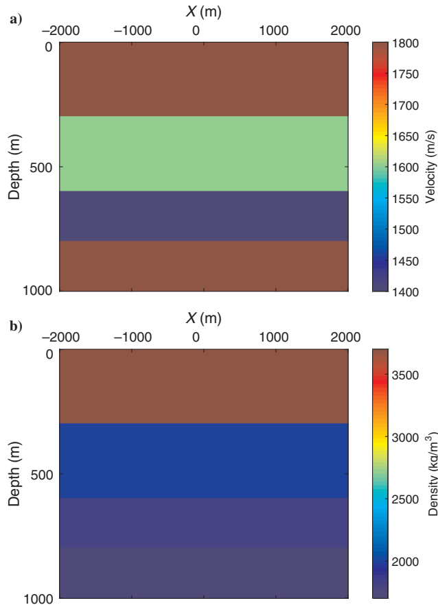
Figure 3. (a) The velocity and (b) density values of the model.
