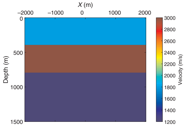
Figure 14. Velocity values of the model.
