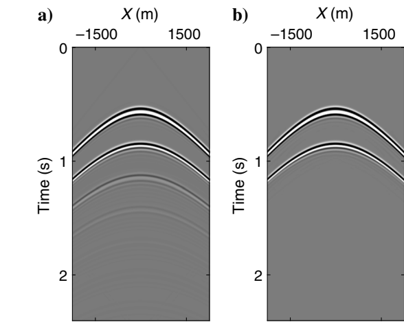
Figure 12. (a) The modeled reflection response and (b) the retrieved data set using equation 21.
