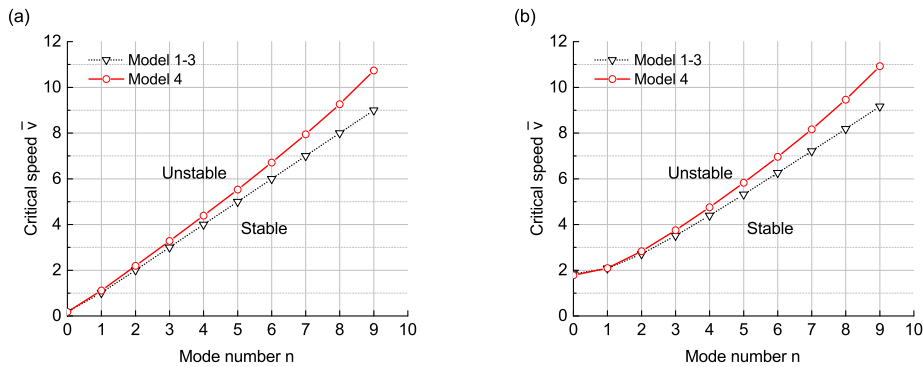
Figure 8: Stability boundaries predicted by different models for h/R = 0.1 , \bar{k}_r = 0.28 : (a) \bar{k}_c/\bar{k}_r = 10^{-4} ; (b) \bar{k}_c/\bar{k}_r = 10^{-2} .
