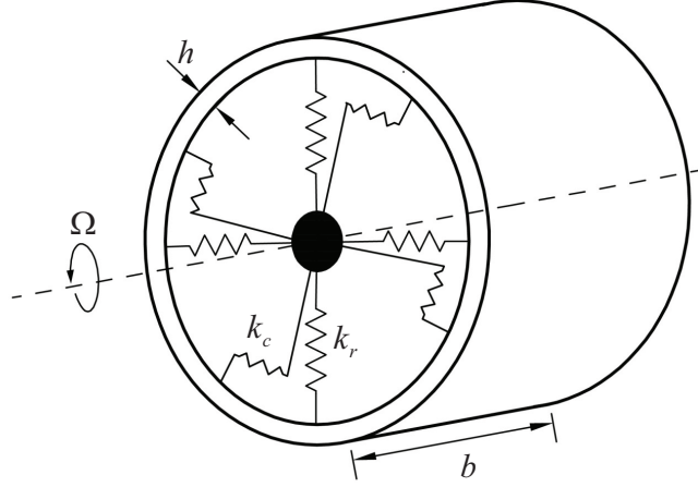
Figure 3: A rotating ring with b \gg h .
