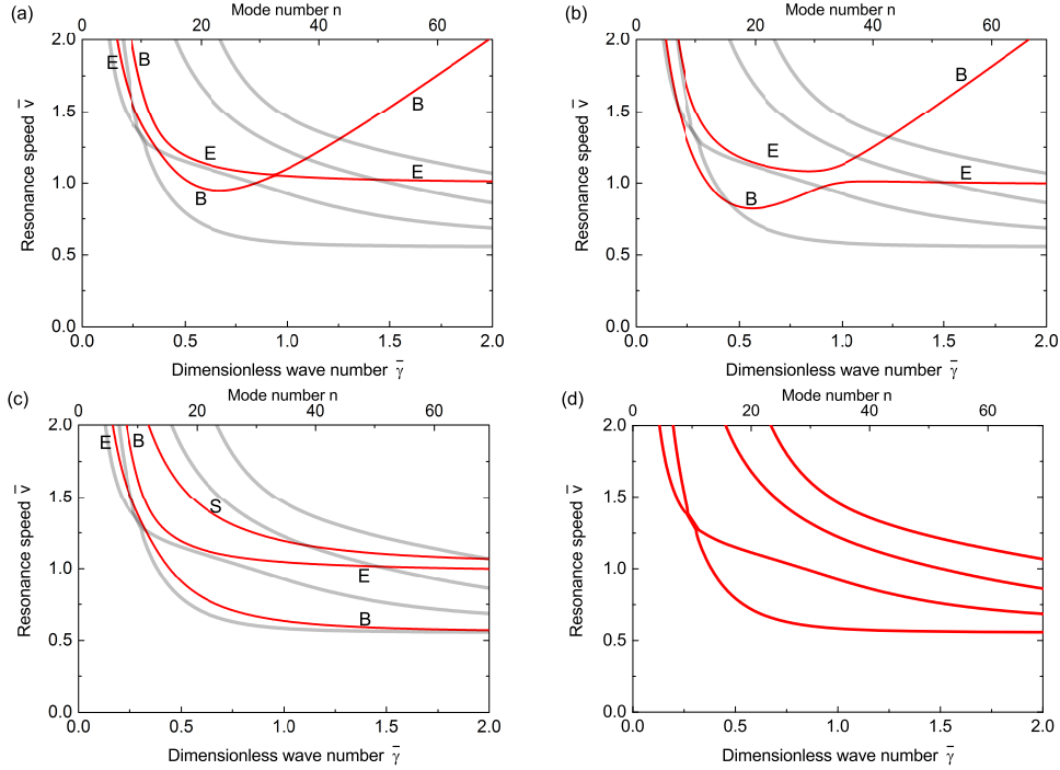
Figure 6: Resonance speeds for h/R = 0.1, \bar{k}_c = 0.1, \bar{k}_r = 0.2 : (a) Model 1 (classical model [13]); (b) Model 2 [22]; (c) Model 3 (Timoshenko-type [18]); (d) Model 4 (the present model).
