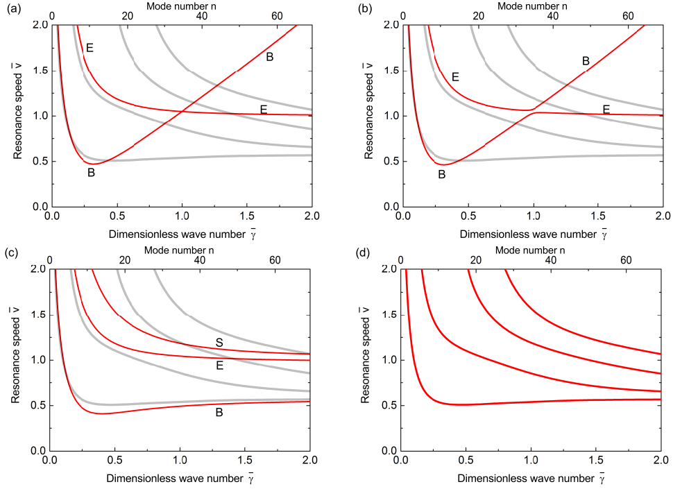
Figure 5: Resonance speeds for h/R = 0.1, \bar{k}_c = 0.1, \bar{k}_r = 0.01 : (a) Model 1 (classical model [13]); (b) Model 2 [22]; (c) Model 3 (Timoshenko-type [18]); (d) Model 4 (the present model).
