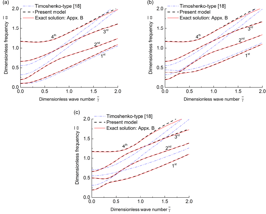
Figure 4: Dispersion curves (plane strain) for h/R = 0.1 , \bar{k}_c = 0.1 and \Omega = 0 : (a) \bar{k}_r = 0.01 ; (b) \bar{k}_r = 0.2 ; (c) \bar{k}_r = 0.5 .
