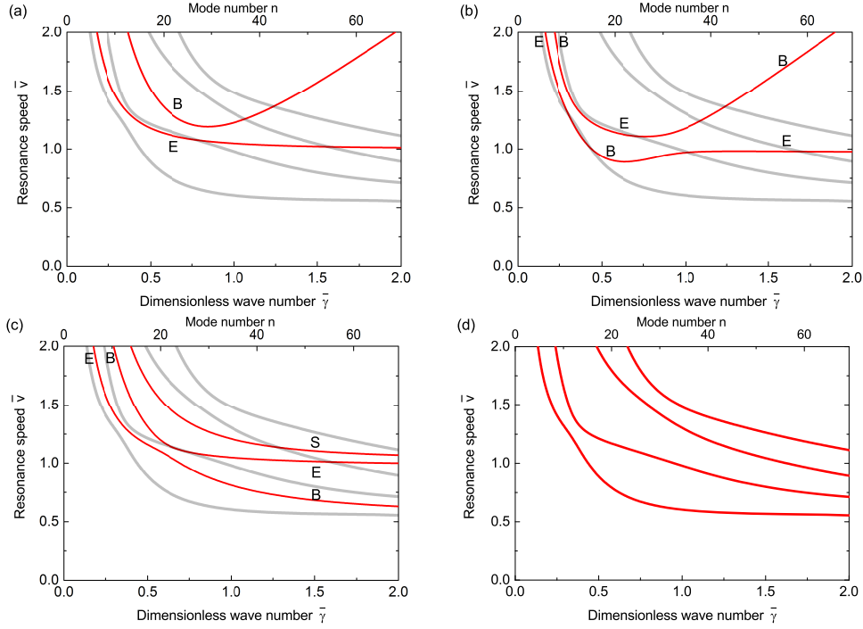
Figure 7: Resonance speeds for h/R = 0.1, \bar{k}_c = 0.1, \bar{k}_r = 0.5 : (a) Model 1 (classical model [13]); (b) Model 2 [22]; (c) Model 3 (Timoshenko-type [18]); (d) Model 4 (the present model).
