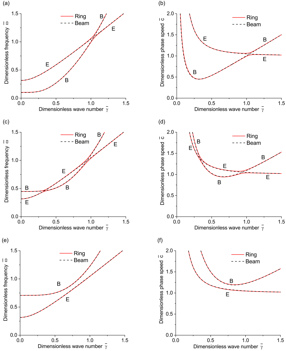
Figure 2: Frequency-wavenumber (left) and phase speed-wavenumber (right) dependencies for h/R = 0.1, \bar{k}_c = 0.1 : (a)(b) \bar{k}_r = 0.01 ; (c)(d) \bar{k}_r = 0.2 ; (e)(f) \bar{k}_r = 0.5 . Note that the wavenumber ranges in the plots exceed the applicable range of the classical theory. However, the range is kept for the convenience of explanation.
