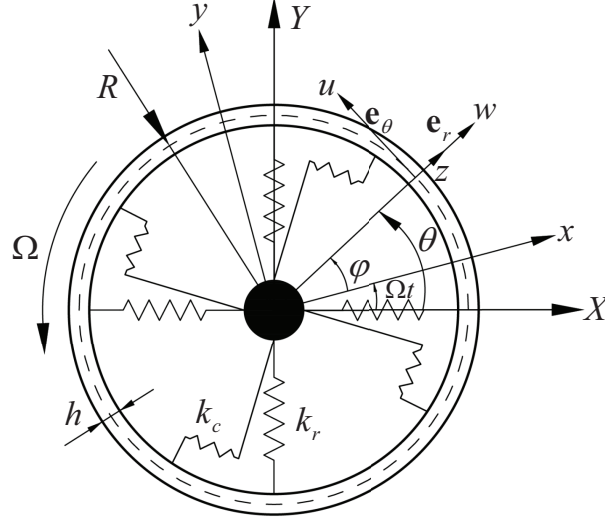
Figure 1: A rotating ring on an elastic foundation
