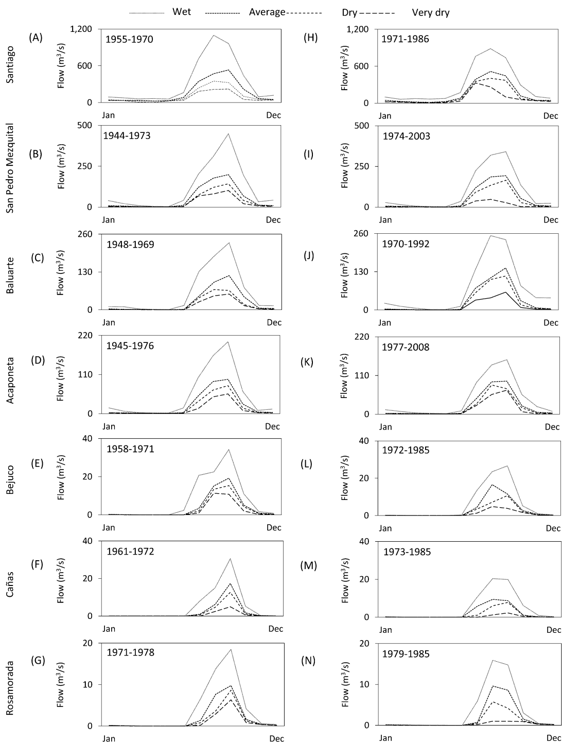
Figure 3.4. Reference (A – G) and assessment (H – N) low flows for wet, average, dry and very dry conditions (monthly scale) of the rivers discharging into Marismas Nacionales wetland.
