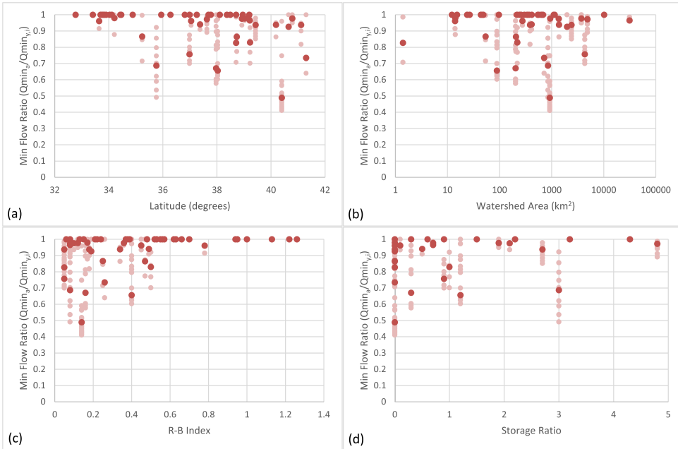
Figure 2.10: Scatter plots of Minimum Flow Ratio as a function of (a) Latitude (decimal degrees), (b) Watershed Area (km 2 ), (c) Richards-Baker Flashiness Index (R-B Index), and (d) Storage Ratio. Average data for all 50 sites shown in dark red; data for all 50 iterations shown in light red. Storage Ratio calculated as the upstream usable reservoir storage divided by the mean annual runoff for the study period. Data shown for the daily subsample interval only.
