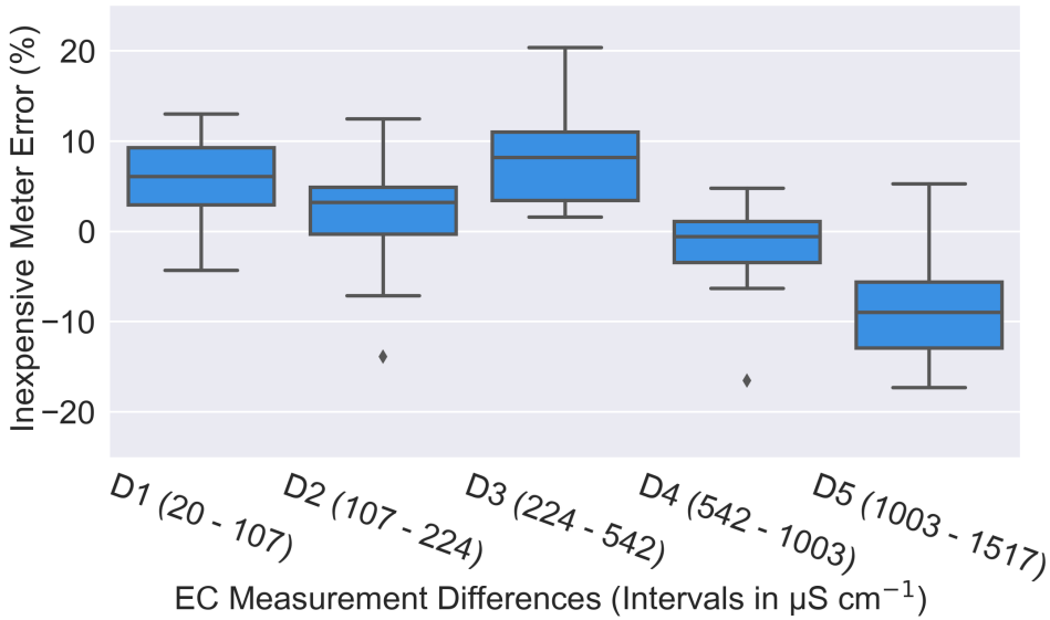
Figure 3.1: Box plots of inexpensive Water Quality Testers [HoneForest] errors for five different intervals (i.e. D1 to D5). The range of EC values from reference EC measurements (determined by a calibrated GHM 3431 [GHM-Greisinger] EC meter) are shown in parentheses in \mu\text{S cm}^{-1} . Boxes show the interquartile range between the first and third quartiles of the dataset, while whiskers extend to show minimum and maximum values of the distribution, except for points that are determined to be "outliers" (shown as diamonds), which are more than 1.5 times the interquartile range away from the first or third quartiles.
