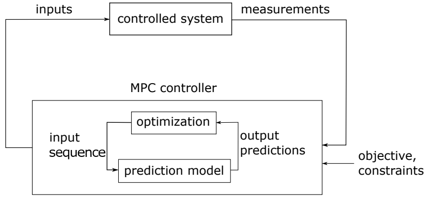
Figure 2.2: MPC loop
