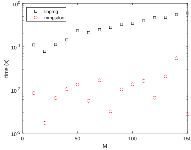
Figure 5.3: CPU time of linprog and optimistic optimization ( mmipsdoo ) for the optimization of MMPS functions ( M is the number of max and min operations of MMPS functions)
