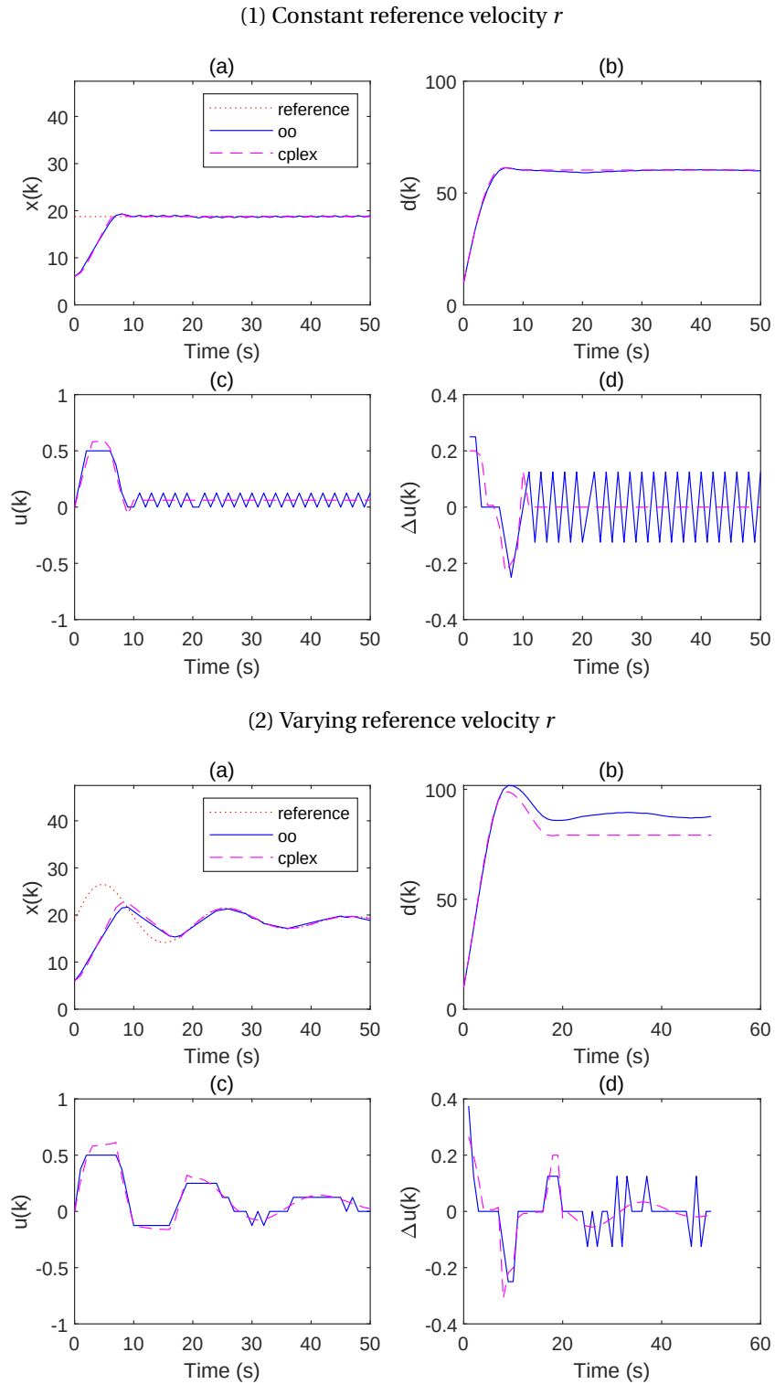
Figure 4.2: Simulation results of cplex and optimistic optimization ( oo ) for the example of Section 4.4 for constant and varying reference velocities ( t_{\max} = 10 for oo ): (a) Velocity of the follower vehicle; (b) Distance between the two vehicles; (c) Control input; (d) Throttle/Brake variation
