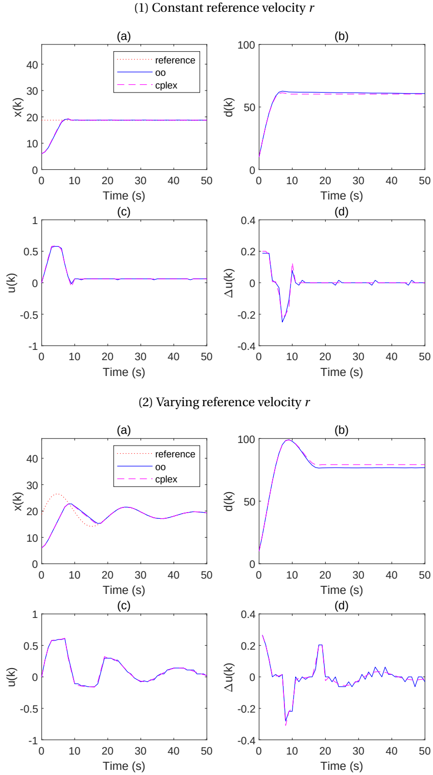
Figure 4.3: Simulation results of cplex and optimistic optimization ( \circ\circ ) for the example of Section 4.4 for constant and varying reference velocities ( t_{\max} = 100 for \circ\circ ): (a) Velocity of the follower vehicle; (b) Distance between the two vehicles; (c) Control input; (d) Throttle/Brake variation
