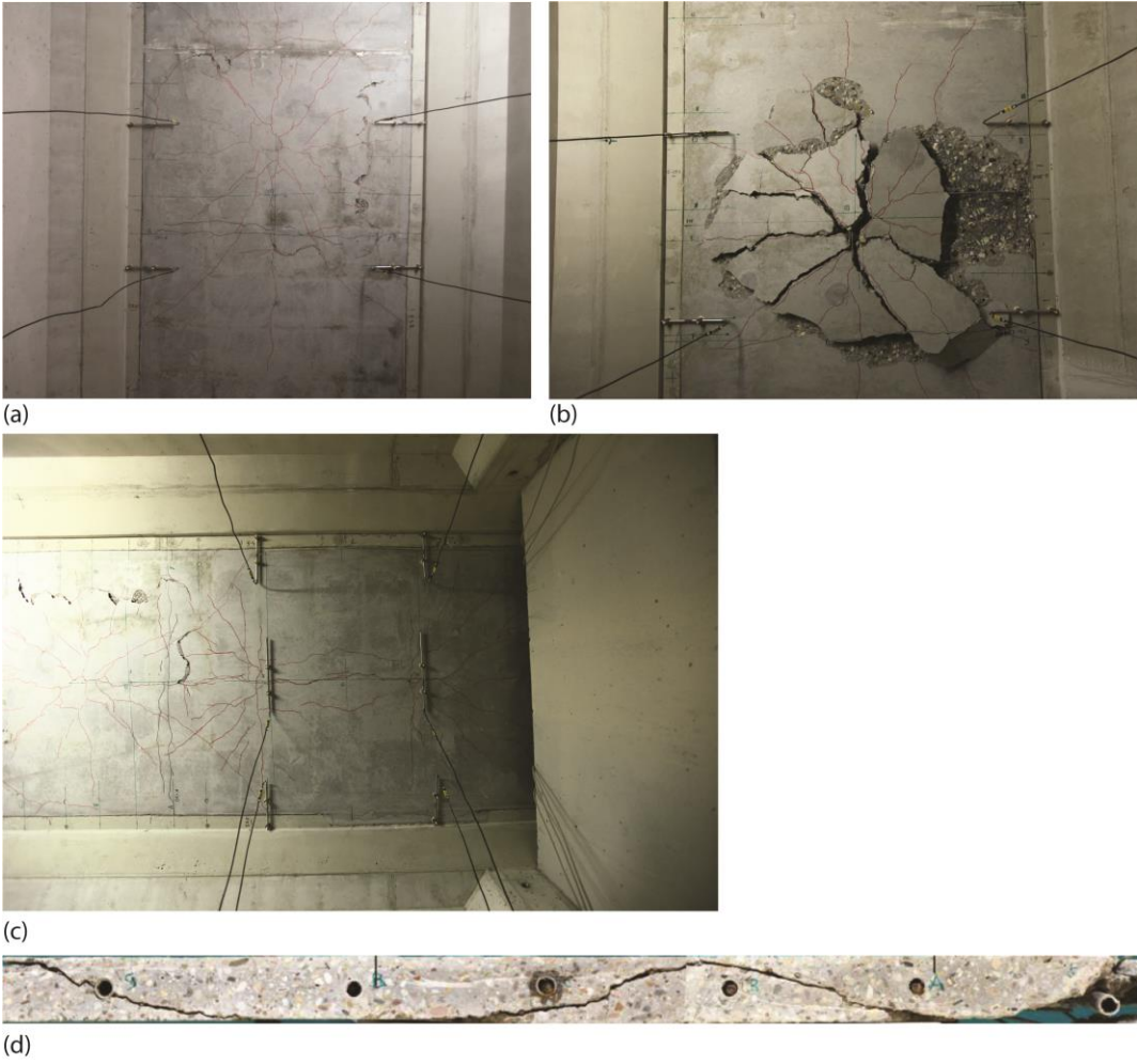
Fig. 5–Specimen after failure: (a) static test BB25, (b) fatigue test BB26 with punching through of load plate, (c) fatigue test BB30 with double wheel print, (d) saw cut of deck showing the ducts of prestressing bars 26 – 30 (right to left) and punching cone of BB27.
