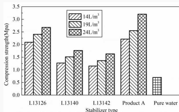
Figure 6: UCS values after 28 days curing.
