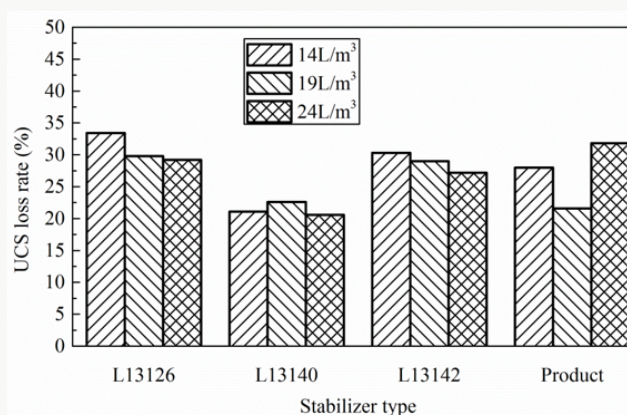
Figure 7: UCS soaked loss rate after 28 curing days.
