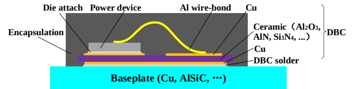
Figure 1. Conventional packaging scheme for a power module
