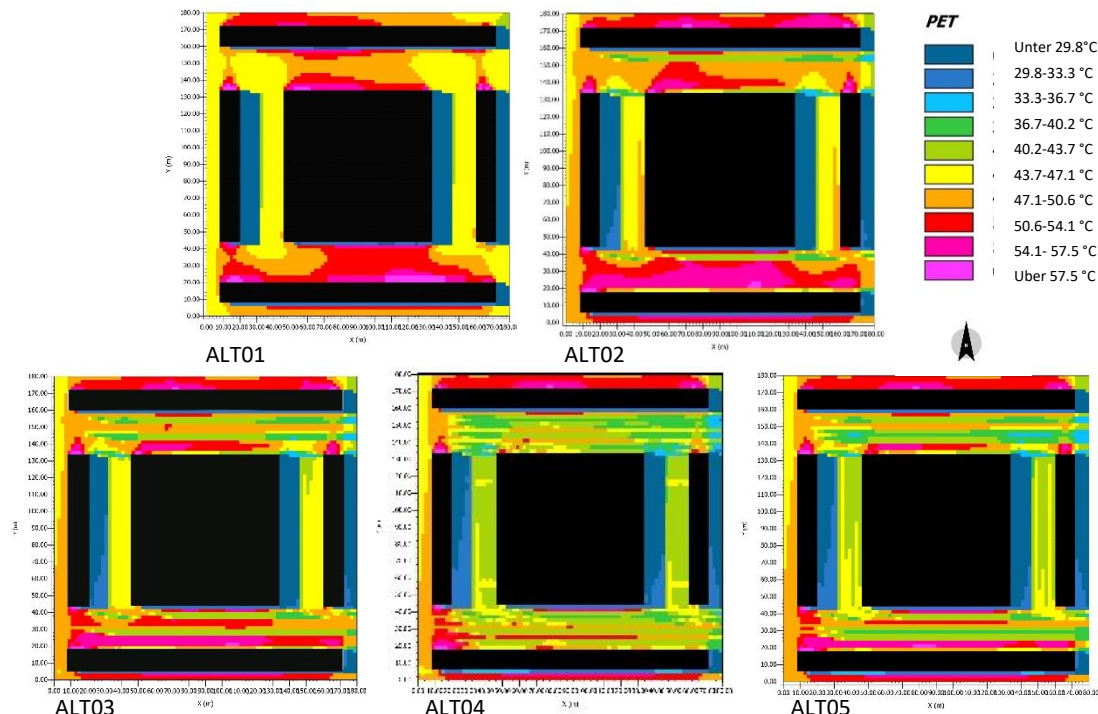
Figure 10: An example of PET simulations by ENVI-met in 13:00 (figures are generated by Leonardo, a component of ENVI-met).
