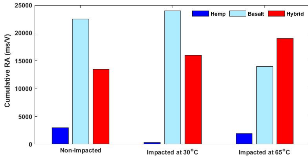
Fig. 11: Comparison of cumulative RA for non-impacted and impacted samples at different temperatures
