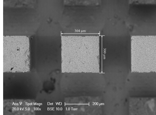
Figure 2: ESEM image of the cross-sections of beams.
