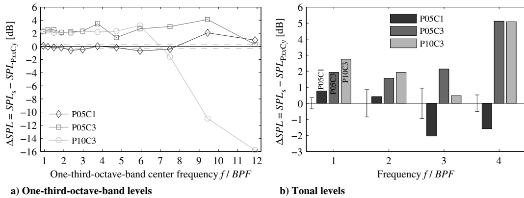
Fig. 23 Reduction in far-field acoustic pressure with respect to the solid pylon, obtained from source power integration in sector II of Fig. 8; Re_c = 550,000 .
