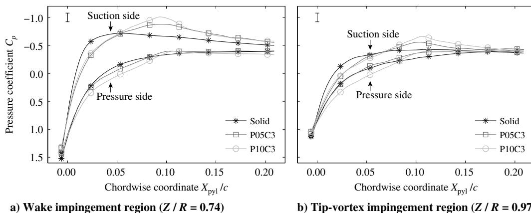
Fig. 16 Pressure distributions around the leading-edge inserts at 0.0075c from the surface; \alpha = 0 deg, Re = 550,000 .
