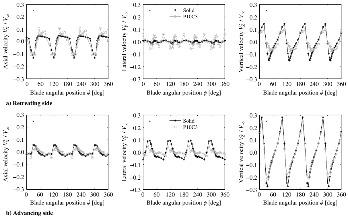
Fig. 19 Velocity fluctuations at 0.0375c from the pylon surface at X_{pyl}/c = 0.08 (i.e., at the markers indicated in Fig. 18); Z/R = 0.97 , \alpha = 0^\circ , Re_c = 550,000 .
