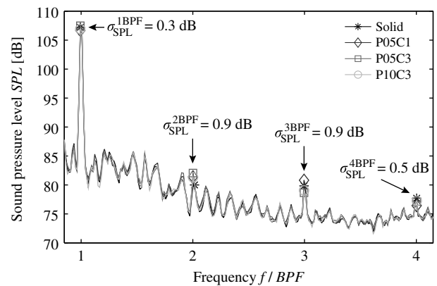
Fig. 22 Narrowband propeller noise spectra obtained from source power integration in sector I of Fig. 8; Re_c = 550,000 .
