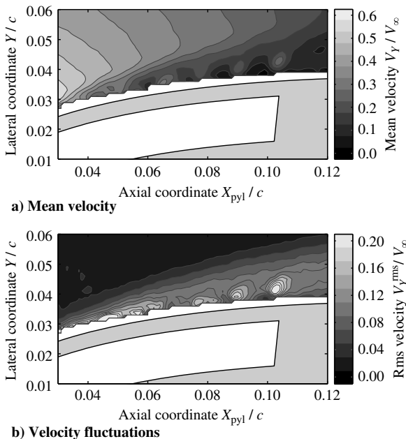
Fig. 11 Lateral velocity component ( Y direction) on the suction side of the P10C3 insert; \alpha = 6 deg, propeller off, Re_c = 550,000 .
