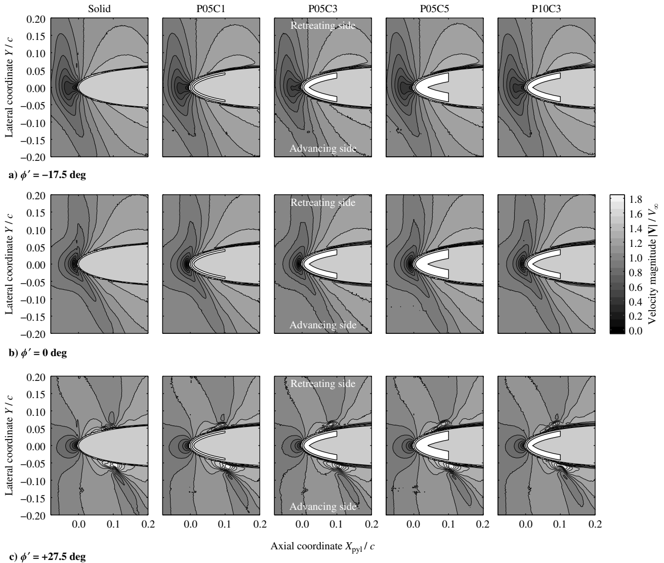
Fig. 17 Velocity fields before, during, and after impingement of the tip vortex on the pylon leading edge; Z/R = 0.97 , \alpha = 0^\circ , Re_c = 550,000 .
