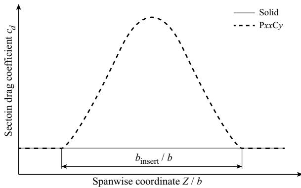
Fig. 6 Determination of spanwise extent of the pylon affected by the flow-permeable insert, based on typical measurement data for the sectional drag.
