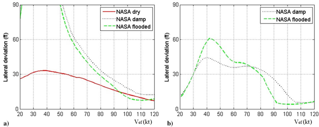
Fig. 12 Lateral deviation as function of V_{\text{eff}} . RTO, NWS on, and 20 kt crosswind with different runway friction models: a) no braking, and b) differential braking.
