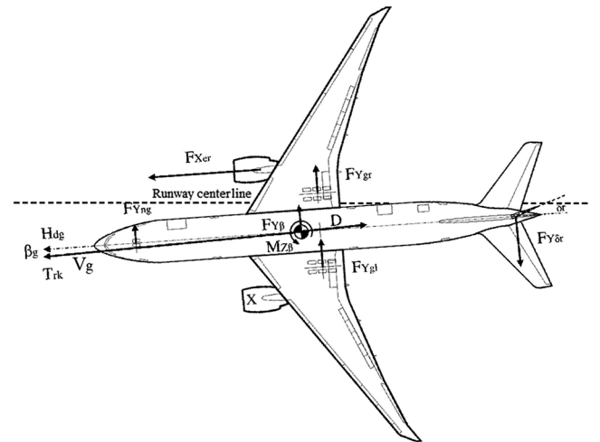
Fig. 4 Situation after rudder application.
