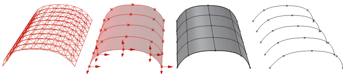
Figure 10. Process of parametric frame structure.
