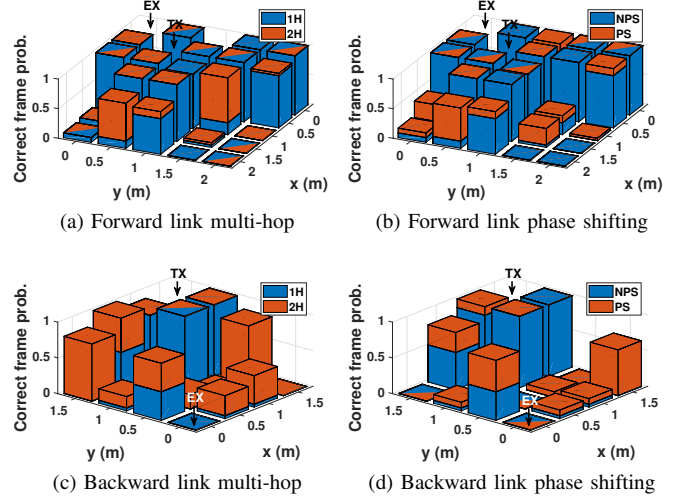
Fig. 10. Backscatter T2T network phase cancellation experiment. EX and TX mark the positions of the exciter and transmitter, respectively. (N)PS: (no) phase shifting. Fig. 10a and 10b: forward link. Both methods yield comparable results. Fig. 10c and 10d: backward link. Multi-hop is superior in network coverage. Note: 1H and NPS is the same case.
