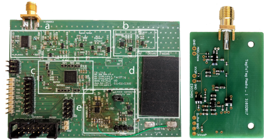
(a) Standalone backscatter T2T tag (b) T2T transceiver
