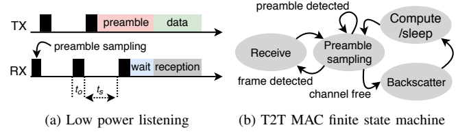
Fig. 7. Schematic representation of the proposed MAC protocol. Fig. 7a: low-power listening diagram (for t_s and t_o see Table IV); Fig. 7b: MAC state machine (for both transmitter and receiver).
