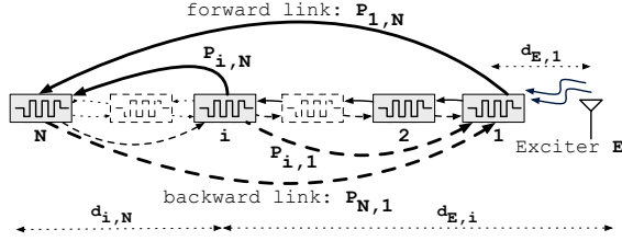
Fig. 3. Multi-hop T2T received power analysis scenario.
