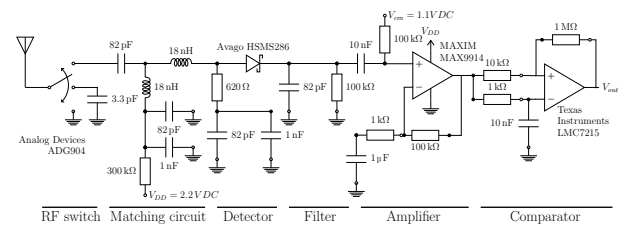
Fig. 6. Backscatter T2T transceiver; its implementation is shown in Fig. 1b.
