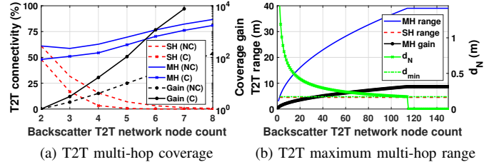
Fig. 4. Backscatter T2T network numerical example with simulation parameters listed in Table II. Fig. 4a: multi-hop versus single-hop full connectivity (probability that all nodes are connected with each other, either only directly, SH, or through hop, MH) with and without phase cancellation; Fig. 4b: multi-hop maximum range in one-dimensional T2T network; NC: no phase cancellation, C: phase cancellation, MH: multi-hop, SH: single-hop.
