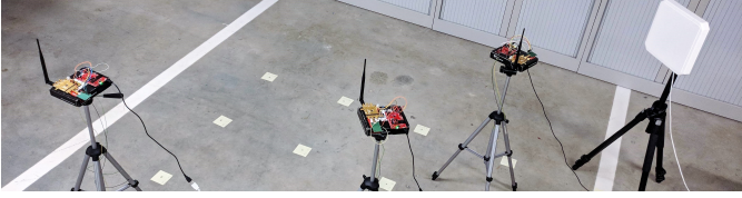
Fig. 9. Photograph of the setup to evaluate phase cancellation countermeasures in T2T networks, discussed in Section VII-C: Three backscatter T2T tags on tripods, next to white panel antenna; grid coordinates marked with yellow squares on the floor.
