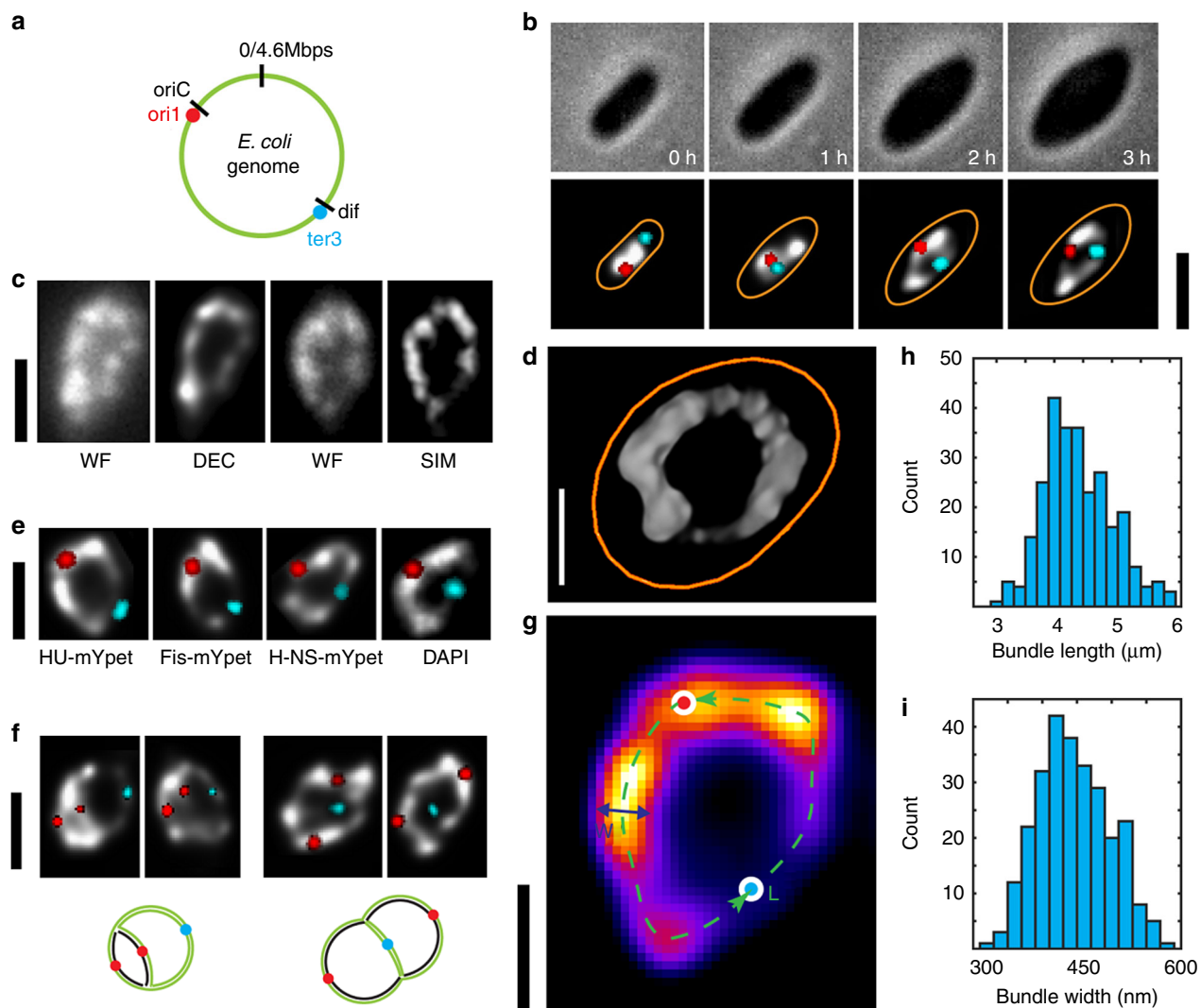
Fig. 1 The circular E. coli chromosome exhibits a toroidal donut-shape that can be visualized upon cell expansion. a Schematic of a E. coli genome. Two FROS markers are shown in red (OriI marked by lacO arrays, targeted by LacI-mCherry) and cyan (Ter3 marked by tetO arrays, targeted by TetR-mCerulean). b Time-lapse fluorescence images of an E. coli ( dnaC2(ts) allele) cell growing into a lemon shape at 40 °C under A22 treatment. Top panel, phase contrast image; bottom panel, overlay of Ori focus (red) and Ter focus (cyan) on a grey-scale deconvolved image of the chromosome labeled by HU-mYPet. Time is indicated in hours. c Fluorescence images showing two opened circular chromosomes captured by different methods. Left: WF, wide-field image, and DEC, deconvolved image of that WF. Right: WF and SIM, structured-illumination microscopy image of that WF image. d Donut-shape chromosome of E. coli , as imaged in 3D-reconstructed SIM. Orange outlines the cell contour. e Similar donut-shape chromosome images are obtained for different DNA-binding fluorescent labels (HU-mYPet, Fis-mYPet, H-NS-mYPet, DAPI; all DEC images). f Fluorescence images of early (left) and late (right) stages of DNA replication of circular chromosomes. Bottom: cartoon illustrations; black strands indicate newly replicated DNA. g Fluorescent image of a donut-shape E. coli genome shown as a heat map. Indicated are the ridge of the bundle (green dashed line), the oriC and dif genomic loci near the origin and terminus of replication (red and blue dots respectively), and the bundle width (blue line). h Histogram of chromosome bundle lengths measured along the bundle ridge (cf. panel G). n = 269 . i Histogram of the average chromosome bundle widths quantified as the full-width-at-half-maximum of the peak intensity across the donut chromosomes. n = 269 . Scale bars in B/C/E/F, 2 \mu\text{m} . Scale bars in D/G, 1 \mu\text{m}
