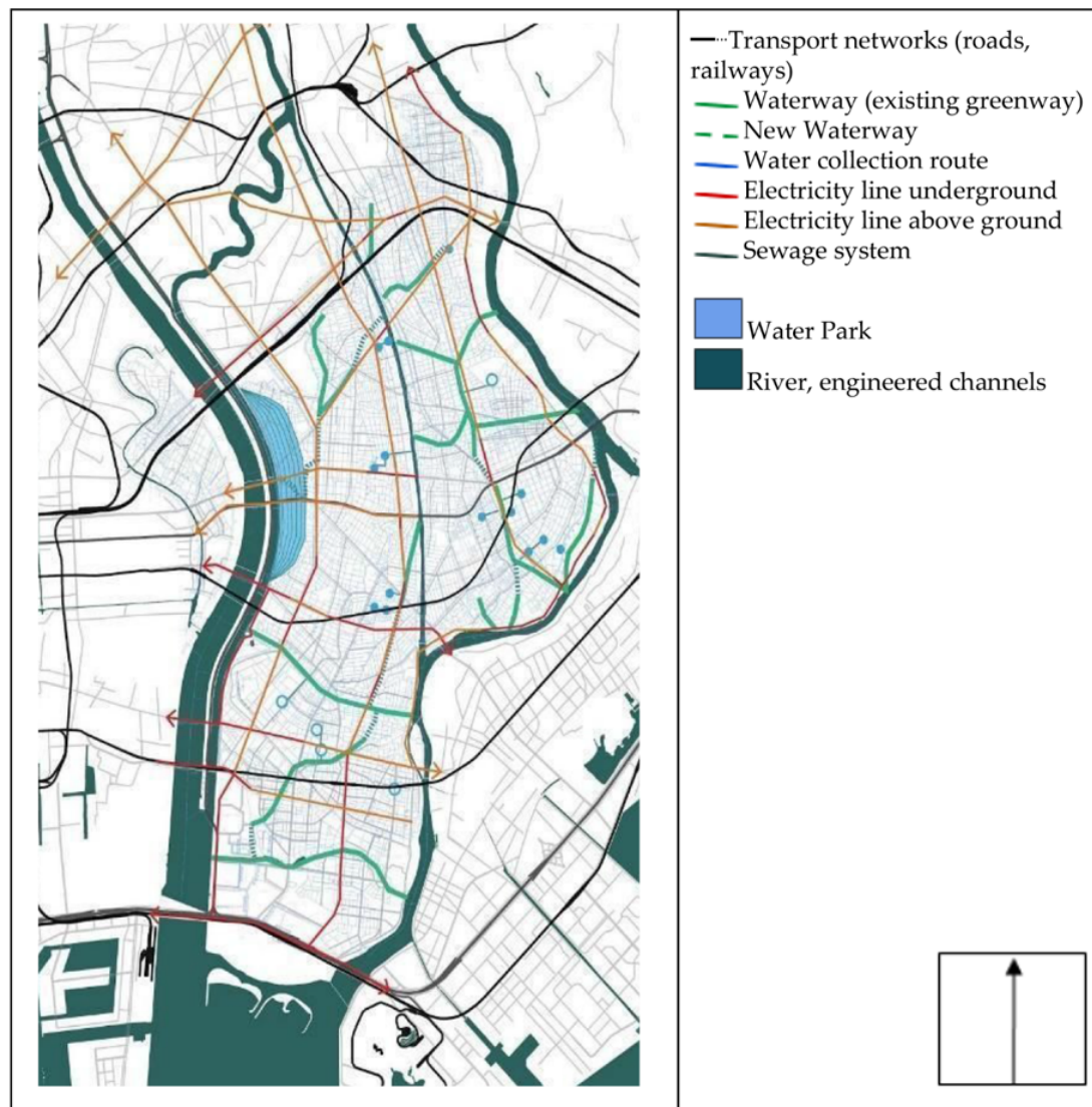
Figure 12. Strategy A—anti super levee overlaid with vital infrastructure (electricity, transport, sewage) (source: drawn using data from MLIT Japan and the Edogawa ward data, 2016) [11,19].
