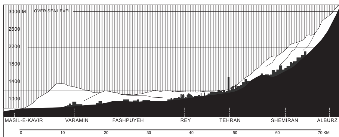
Figure 1.2 Tehran Topography
