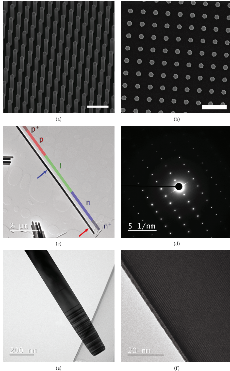
FIGURE 1: SEM and TEM of selective area InP nanowires. (a) SEM image, inclined 30^\circ respective to the normal, of SA i-InP. The scale bar is 1\ \mu\text{m} . (b) Top view SEM image of i-InP nanowires taken normal to the substrate. The scale bar is 1\ \mu\text{m} . (c) Overview of a bright-field TEM image of a representative nanowire with a p^+ - p - i - n - n^+ doping profile. The nominal design of the doping profile is depicted in the image as well. (d) Selected area electron diffraction pattern, acquired from a 1.3\ \mu\text{m} -long segment of the middle part of the nanowire, displaying the wurtzite structure. (e) BF-TEM image of the top of the wire (red arrow panel (c)), displaying the defected top n^- -doped part and the defect-free rest of the NW. (f) HRTEM image of the center of the nanowire (blue arrow panel (c)), displaying the perfect wurtzite structure.
