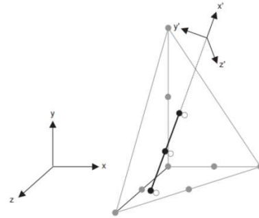
Figure 1. Embedded beam element in PLAXIS 3D as presented by Brinkgreve et al. (2015)
