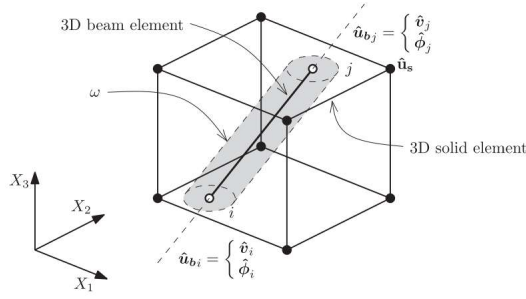
Figure 2. Embedded beam element as proposed by Turrello et al. (2016a)
