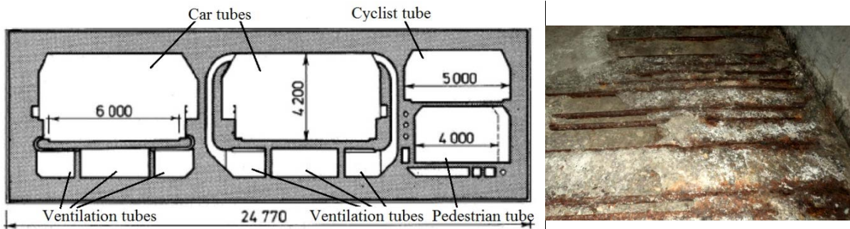
Figure 17: The Maastunnel a) Cross section of the tunnel b) chloride induced corrosion damage in ventilation tubes.
