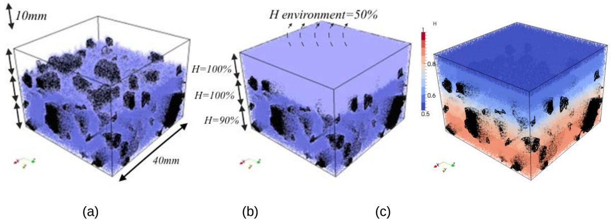
Figure 12: Restrained shrinkage induced damage in the repair system simulated by the lattice moisture model and lattice fracture model a) imitating "sandblasted" surface roughness of the substrate, b) "Casting" repair material and "exposing" it to drying, c) moisture profile after 110 days of drying.
