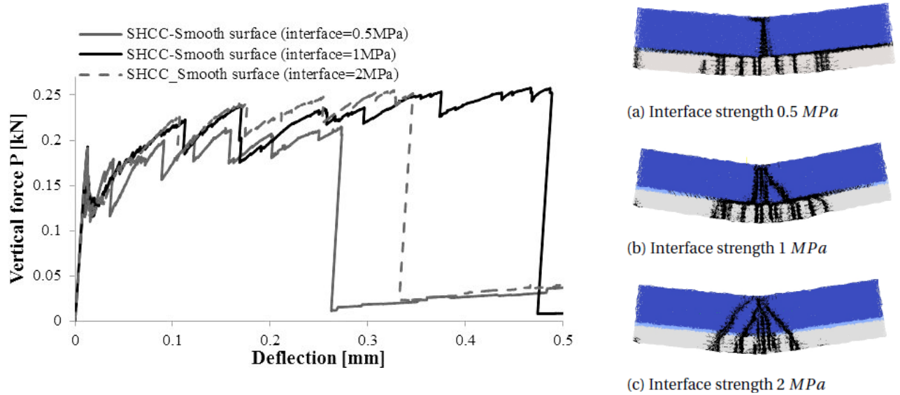
Figure 9: Force-deflection diagram in three-point bending test for different interface strength in smooth surface for SHCC specimens with corresponding final fracture patterns on right
