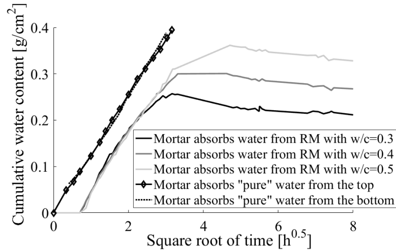
Figure 2: Cumulative moisture absorption by the mortar substrate from Repair Material (RM) with w/c of 0.3, 0.4 and 0.5 in repair systems, compared to cumulative moisture absorption when "pure" water is absorbed from the top or bottom of the mortar.
