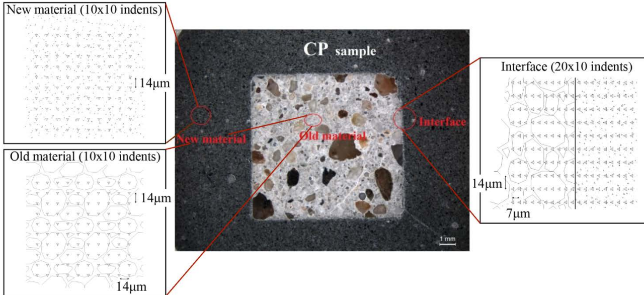
Figure 4: Reflected light photomicrographs of one set of locations for the nanoindentation testing. New material = Cement paste (CP), Old material = Substrate, 5 years old mortar
