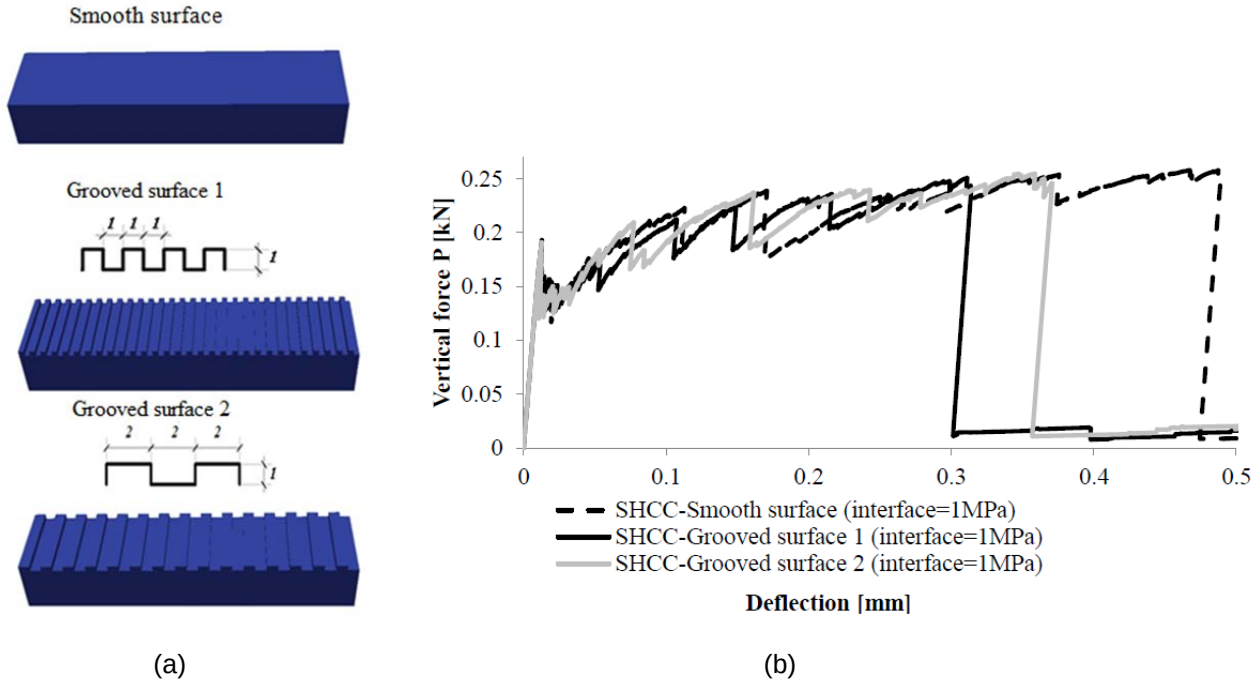
Figure 7: a) Simulated surface profiles b) Force-deflection diagram in three-point bending tests for different roughness profiles for SHCC repair system
