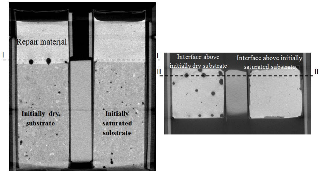
Figure 3: X-ray computed tomography images from repair systems with initially dry and saturated substrate made at the age of 3 days after casting the repair material with w/c of 0.3 (repair material thickness 15 mm, mortar substrate thickness 40 mm).
