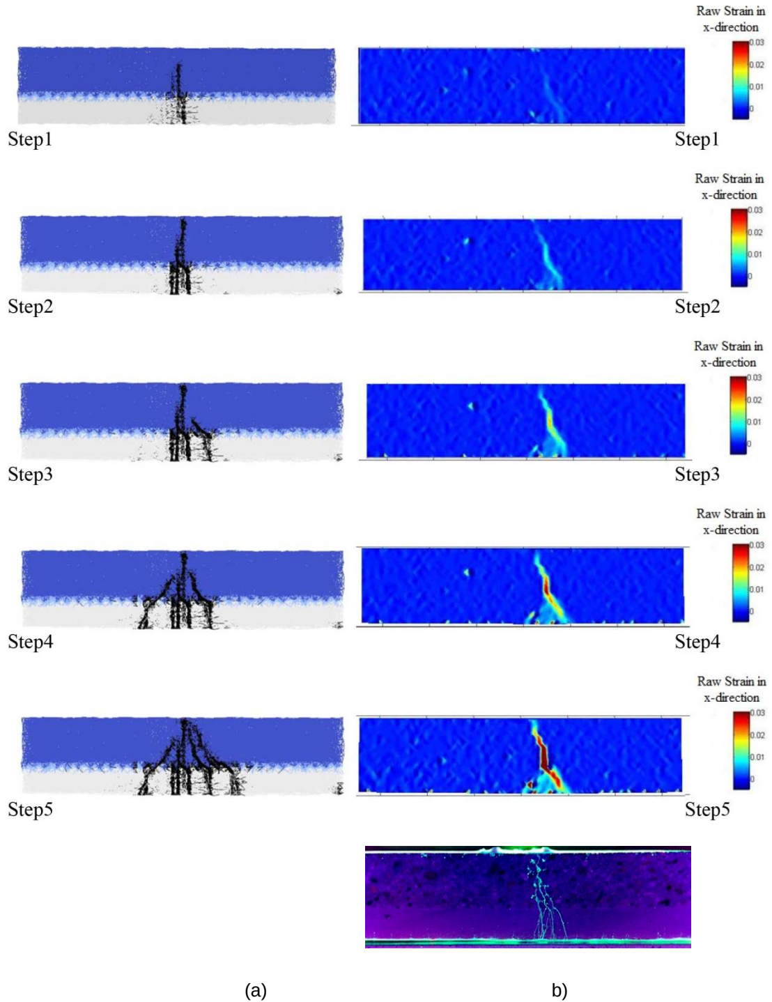
Figure 11: Crack development in different stages of loading in a) simulated and b) tested repair system with the final crack pattern (after testing sample was impregnated with fluorescent epoxy and cut in the middle), top - mortar substrate, bottom - SHCC.
