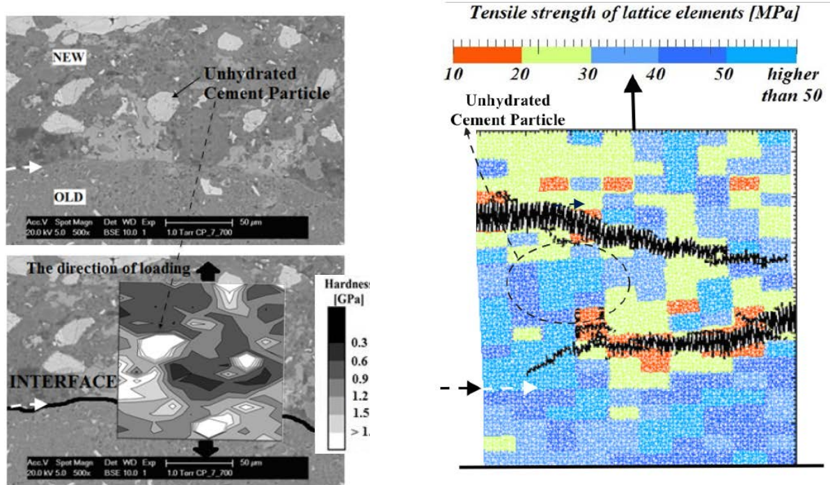
(a) Initial microstructure (top) with the measured hardness (bottom) used as input for lattice modelling
