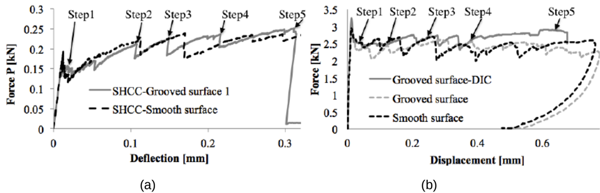
Figure 10: a) Simulated samples and b) Experimentally tested samples (Grooved surface – DIC / the specimen which was processed by DIC technique)
