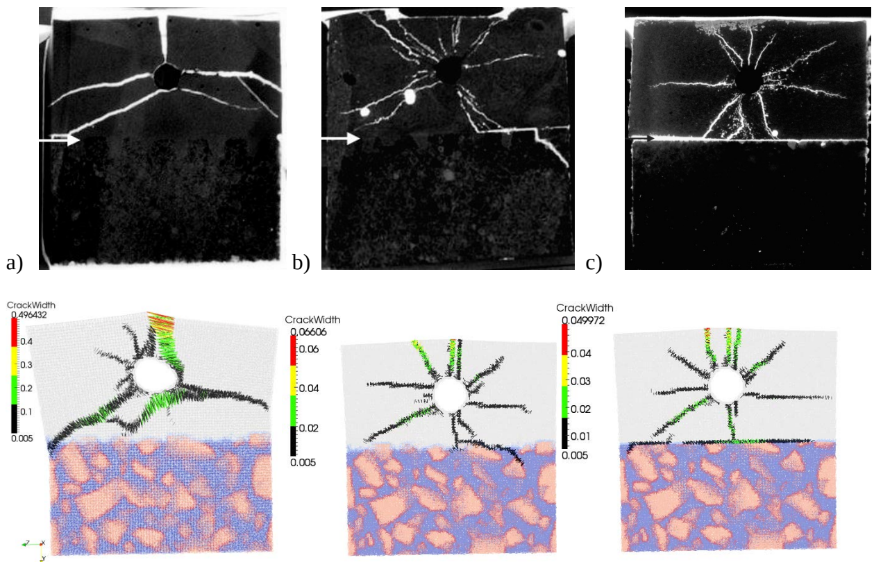
Figure 16: Experimentally (top) and numerically (bottom) obtained crack pattern and maximum crack widths in [mm] due to the pressure imposed by expanding bar in the repair material. a) convention repair material with the rough surface of the substrate; SHCC as a repair material with the b) rough surface and c) smooth surface of the substrate.
