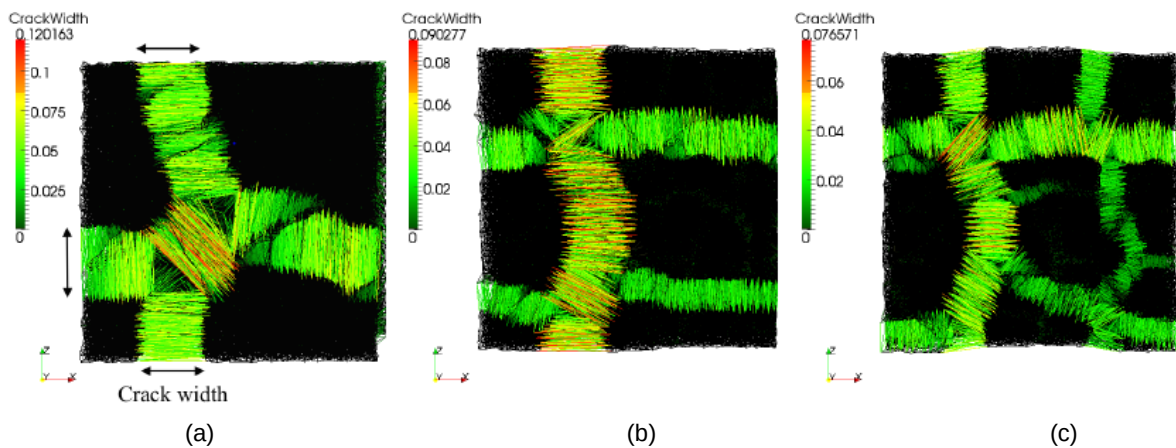
Figure 13 Resulting damage pattern due to restrained shrinkage deformation, influence of bond strength and substrate roughness on cracking after 110 days of drying in a) smooth surface, interface strength 1 MPa, b) rough surface, interface strength 1 MPa and c) rough surface, interface strength 3 MPa.
