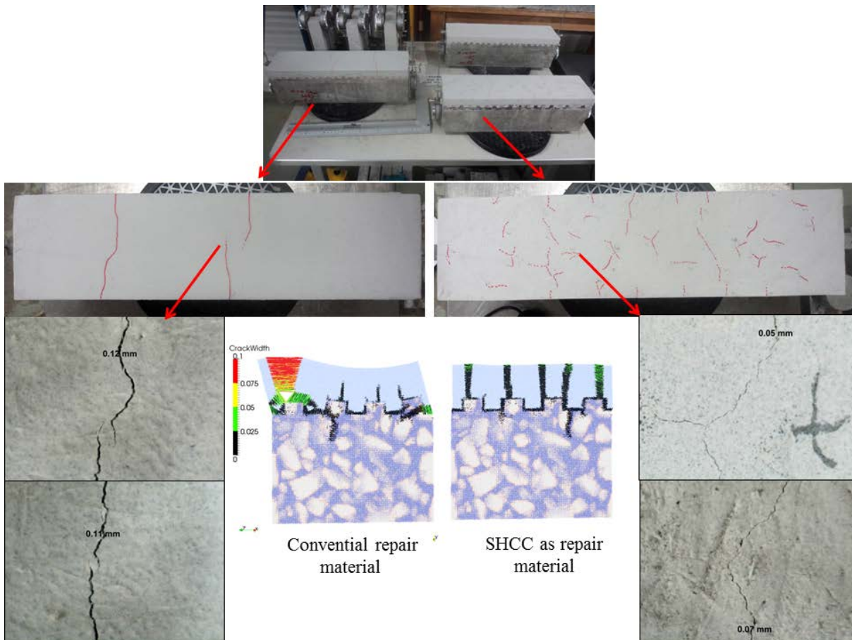
Figure 15: Experimentally obtained damage behaviour compared to numerically simulated in commercial repair material (left) and SHCC (right) with the grooved surface of the substrate.
