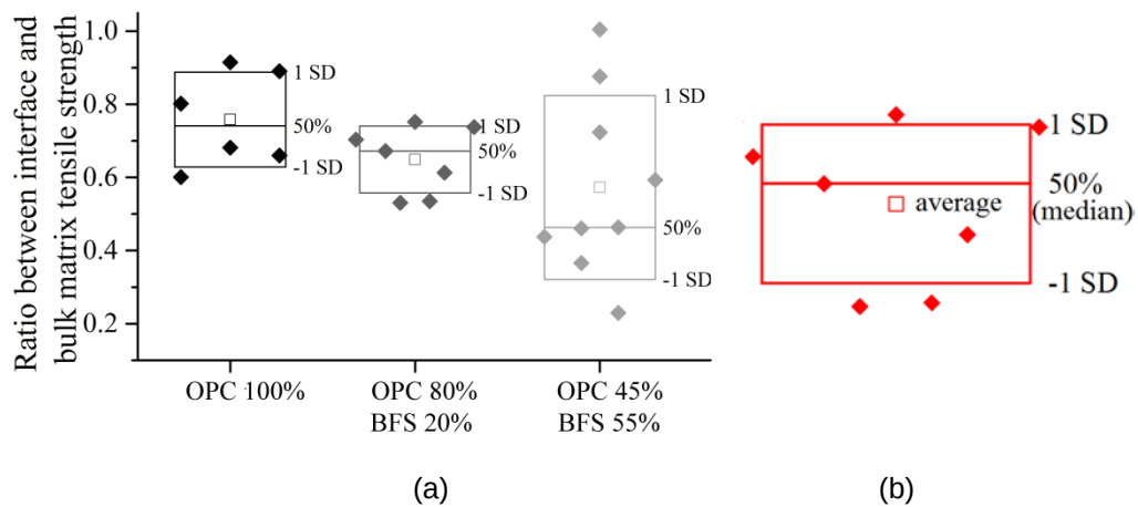
Figure 6: a) Calculated ratio between the tensile strength of interface and tensile strength of repair material for different types of repair materials (percentage given by total binder content), b) legend, SD is standard deviation.
