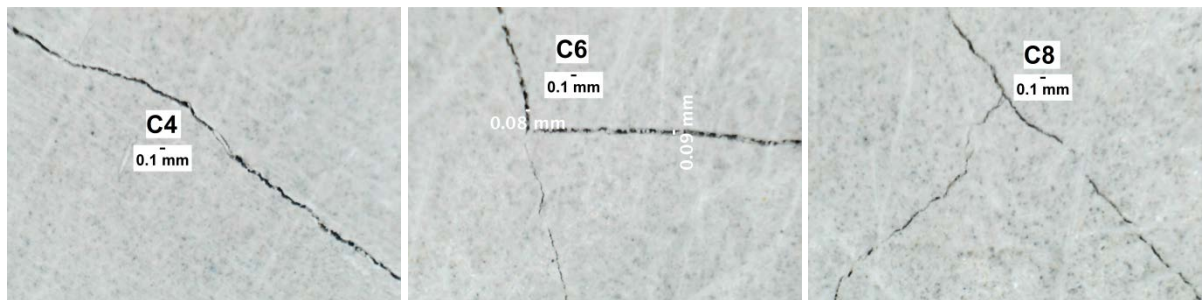
Figure 19: Shrinkage induced cracks in SHCC patch repair and magnified cracks (bottom).
