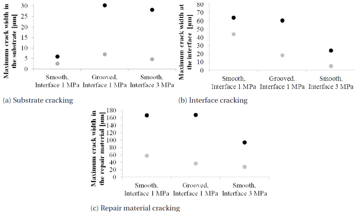
Figure 14: Influence of the substrate roughness and bond strength on the damage in the repair system, black - repair mortar, grey – SHCC.
