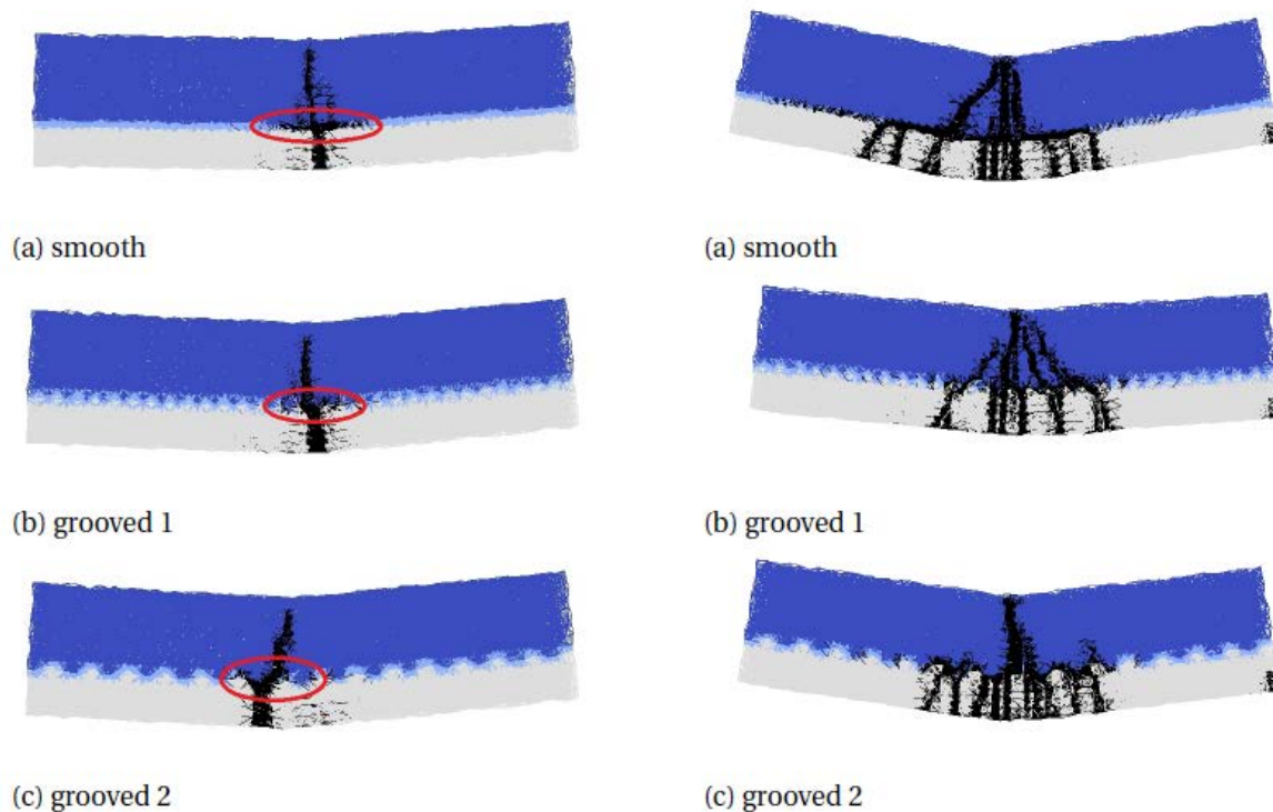
Figure 8: Simulated final fracture pattern in non-fibre reinforced (left) and SHCC (right) repair system
