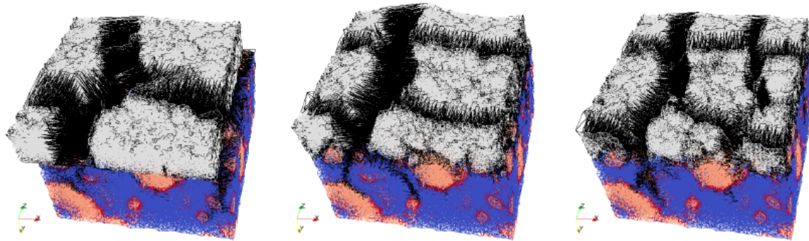
Figure 12: Restrained shrinkage induced damage in the repair system simulated by the lattice moisture model and lattice fracture model a) imitating "sandblasted" surface roughness of the substrate, b) "Casting" repair material and "exposing" it to drying, c) moisture profile after 110 days of drying.
