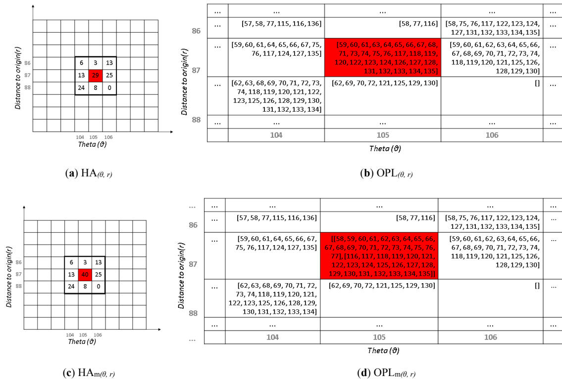
Figure 5. Cells in HA, OPL, HA_m , and OPL_m for r = 86 – 88 and \theta = 104^\circ – 106^\circ . Red cells correspond to hotspots. (a) HA_{(\theta, r)} cell containing accumulated numbers of points voting for a line; (b) OPL_{(\theta, r)} cell containing lists of points voting for the same line; (c) HA_m_{(\theta, r)} cell containing merged accumulated number of points from its adjacent cell; (d) OPL_m_{(\theta, r)} cell containing lists of merged points from its adjacent cell.
