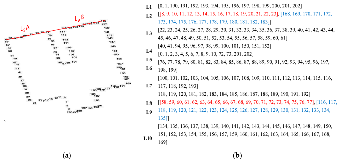
Figure 6. Representation of ordered edge point distribution of a building. Lines are separated in segments by gap identification. (a) Line L9 (red) consists of two segments: L_{9A} and L_{9B} ; (b) List of points supporting the same line. The line points in L2 and L9 are both divided over two segments, indicated by red and blue numbers.
