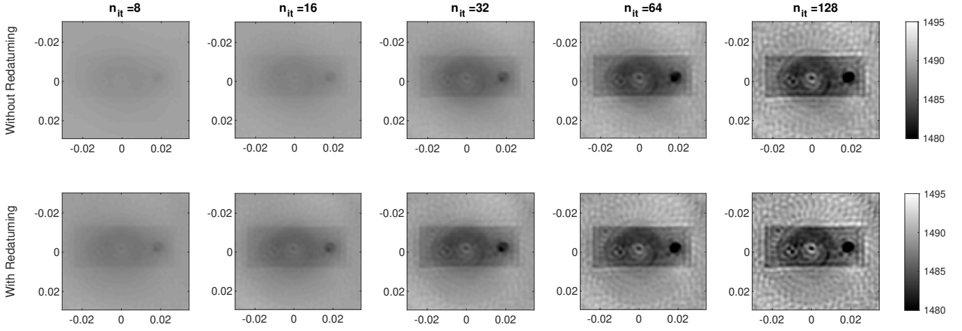
Fig. 10. CSI results before and after redatuming for an increasing number of iterations ( n_{it} = 8, 16, 32, 64 , and 128 ). Note that these results are obtained using the same five frequency components. The gray scale indicates speed of sound values in m/s.
