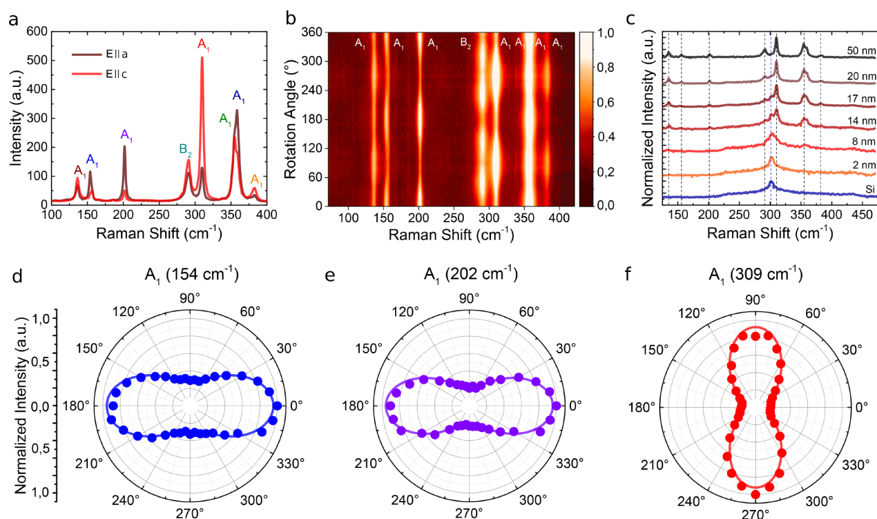
Figure 2. (a) Raman spectra of a bulk \text{As}_2\text{S}_3 crystal (thickness, t \approx 50 nm) for a polarization of incident red laser light ( \lambda = 632 nm) along two crystalline axes ( a and c ). (b) Polarization-dependent Raman intensity spectra obtained by sample rotation with normal incident light (along the b -axis of a crystal). (c) Thickness-dependent Raman spectra under \lambda = 632 nm excitation. (d–f) Polarization dependence for three Raman-active modes. Vibrational modes in a, b, and d–f are labeled in accordance to previous works 40–45 on \text{As}_2\text{S}_3 .
