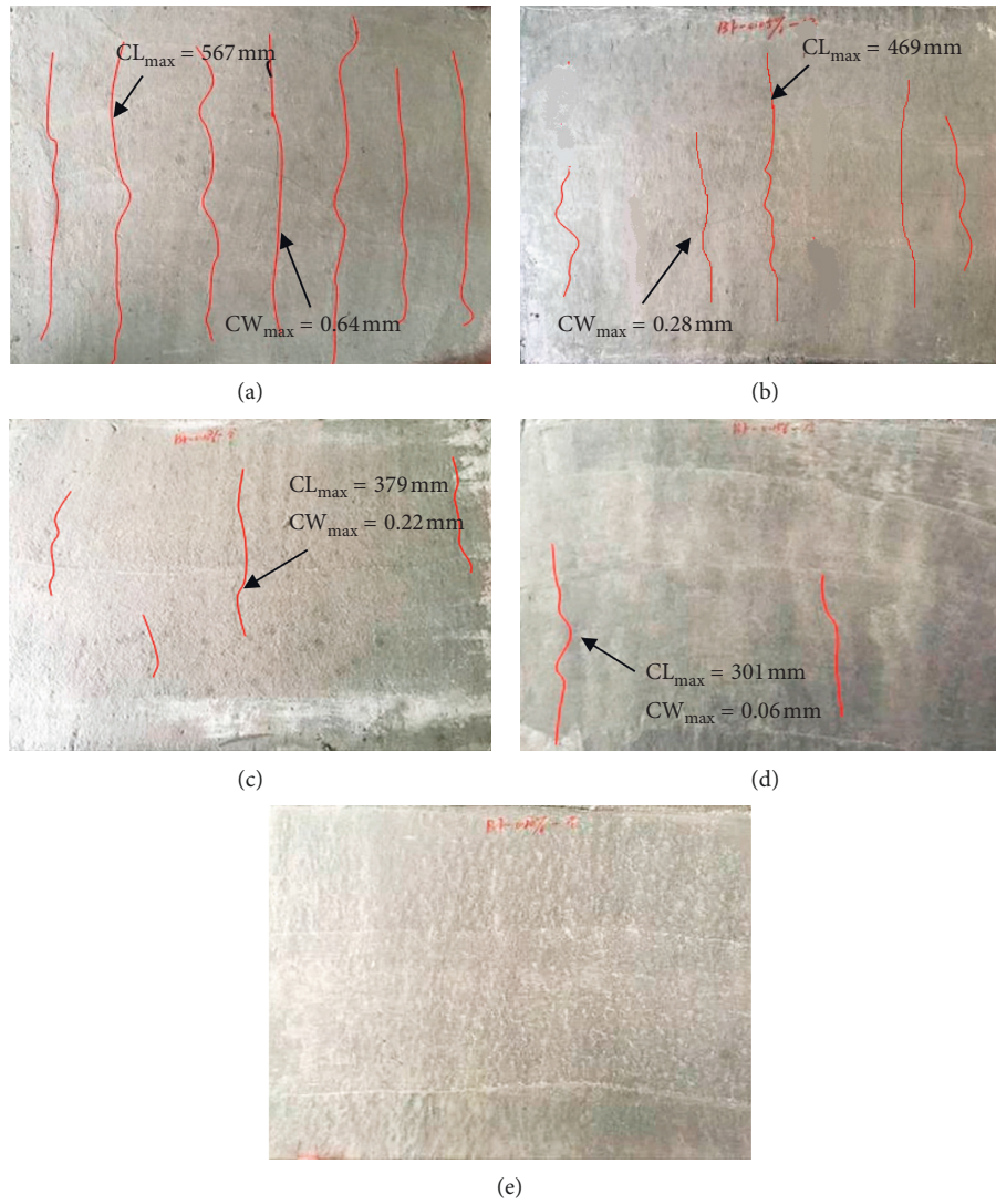
FIGURE 13: The crack distributions of specimens PC30 and BFRC with different fiber volume fractions: (a) PC30 (0%), (b) BF 30-18-0.05 (0.05%), (c) BF 30-18-0.10 (0.10%), (d) BF 30-18-0.15 (0.15%), and (e) BF 30-18-0.20 (0.20%).
