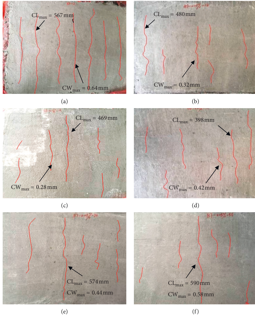
FIGURE 11: Crack distributions of specimens PC30 and BFRC with different fiber lengths: (a) PC30 ( L = 0 mm), (b) BF 30-12-0.05 ( L = 12 mm), (c) BF 30-18-0.05 ( L = 18 mm), (d) BF 30-24-0.05 ( L = 24 mm), (e) BF 30-30-0.05 ( L = 30 mm), and (f) BF 30-36-0.05 ( L = 36 mm).
