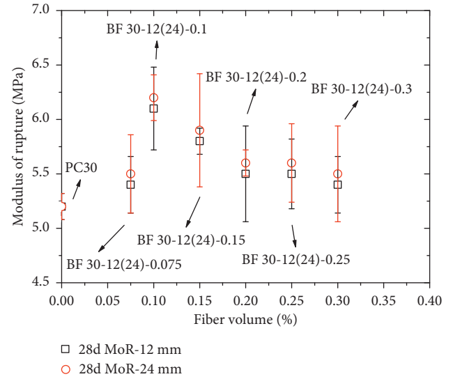
FIGURE 8: Effect of fiber volume fraction on MoR for specimens PC30 and BF 30-12(24)-(0.075~0.3).
