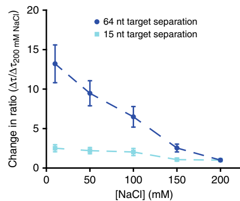
Fig. 6 Argonaute target search is characterized by sliding and intersegmental transfer. The relative change in shuttling time of two constructs from Fig. 3, 64 nt separation (dark blue circles) and 15 nt separation (light blue squares), normalized against \Delta\tau_{\text{shuttle}} at 200 mM NaCl. Errors of the ratio were determined through bootstrapping 10^5 times the ratio of \Delta\tau_{\text{shuttle}}/\Delta\tau_{\text{shuttle}}^{200 \text{ mM NaCl}} . Source data are provided as a Source Data file
