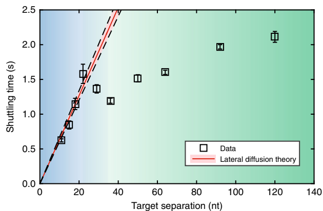
Fig. 3 CbAgo shuttling behaviour differs across short and large distances. Shuttling time is plotted vs. distance between targets. Squares indicate the mean shuttling time for each DNA construct. The plotted error bars indicate the 95% confidence interval of 10^5 bootstrapped dwell times. The red line indicates the lateral diffusion model where the first four datapoints are fitted with k_{\text{esc}} = 15.8 \text{ s}^{-1} . The shaded red region indicates its 95% confidence interval derived from bootstrapping the data. The blue region indicates where the shuttling time follows lateral diffusion theory. This theory breaks down for larger distances (green). Source data are provided as a Source Data file
