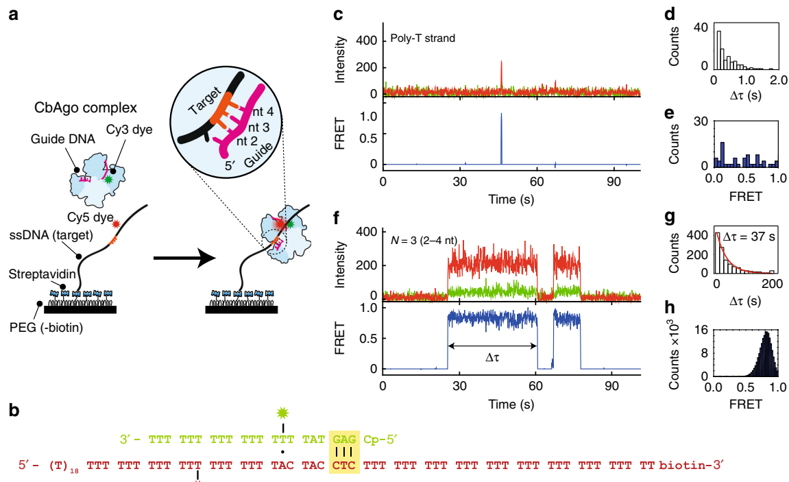
Fig. 1 Single molecule imaging of target binding by siDNA:CbAgo complex. a Immobilization scheme of the Argonaute-guide DNA complex. ssDNA is immobilized on a PEGylated quartz slide surface. Presence of the Ago-siDNA complex is detected by specific binding to target site (light yellow) resulting in high FRET. b Sequences of guide (green) and target DNA (red). Guide is labelled on the 9th nucleotide position from the 5' side. c Representative FRET trace of a single molecule experiment at 100 mM NaCl showing a transient interaction between CbAgo and a poly-T strand. Time resolution is 100 ms. d Dwell time distribution of the Argonaute in absence of target motif. e FRET values of the transient interactions. f Representative FRET trace of a single molecule experiment showing the interaction between CbAgo and a 2-4 nt ( N=3 ) motif. g Dwell time distribution of N=3 binding events with the mean dwell time of 37 s. h FRET histogram of binding events, showing a single FRET population for N=3 at E=0.78 . Source data are provided as a Source Data file
