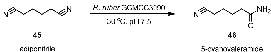
Scheme 14. Nitrile hydratase catalyzed bioconversion of adiponitrile ( 45 ) yielding 5-cyanovaleramide ( 46 ) using whole-cells of R. ruber CGMCC3090 [139].
