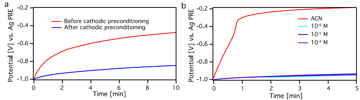
Figure 2. Impurities are reduced in a 0.1 M LiClO 4 acetonitrile (ACN) electrolyte solution. a) Fermi-level stability measurements for a ZnO QD film on an ITO before and after a cathodic preconditioning of -1.0 V was applied to the electrolyte solution (with a bare ITO for two hours). b) Fermi-level stability measurements performed with different concentration of Li[Et 3 BH] ranging from 10 -6 to 10 -4 M. By performing a cathodic preconditioning step or by adding super hydride to the solution, the doping stability increases greatly.
