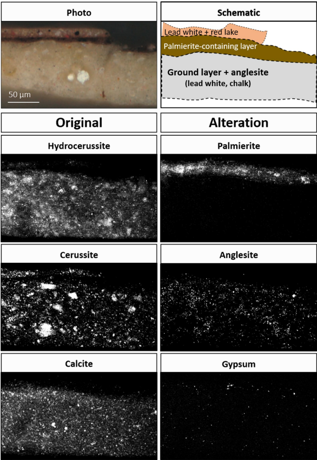
Fig. 4 Results obtained with \mu -XRPD. Distribution images obtained with \mu -XRPD showing the scaling parameter for every pixel. Higher scaling parameters are represented by a brighter colour
