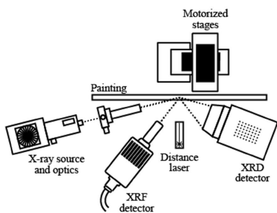
Fig. 1 Schematic and visual photo of the MA-rXRPD scanner
