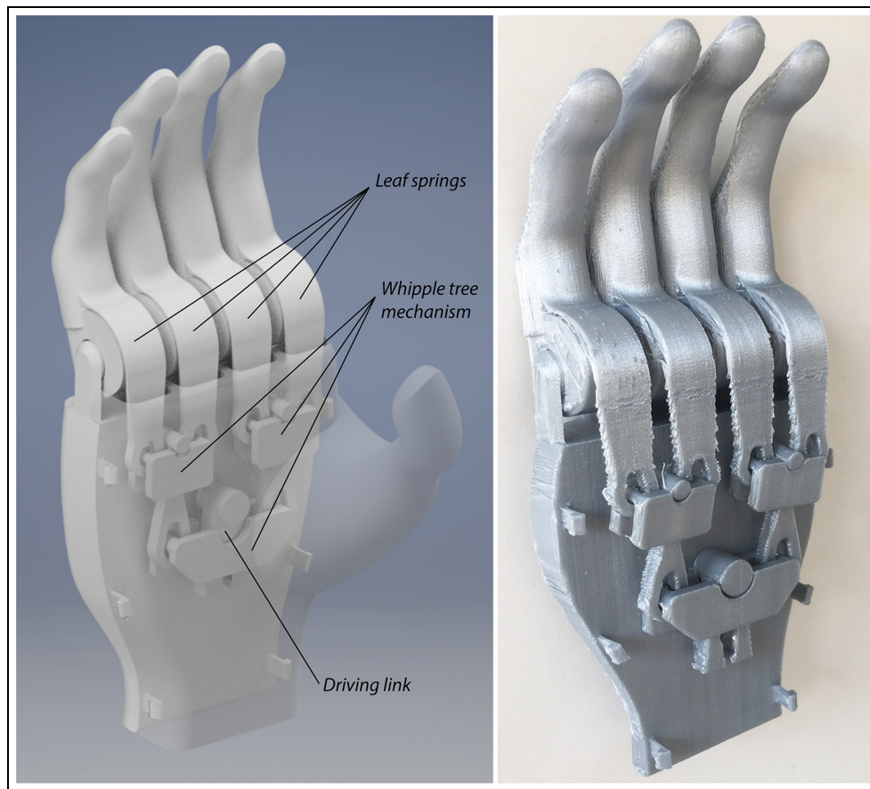
Figure 1. Design of our 3D-printed prosthetic hand. The palm in the left picture is translucent to show the inner mechanisms (from top to bottom: leaf springs, whippletree mechanisms, and driving link), and the right picture shows the 3D-printed prosthetic hand without the palm.
