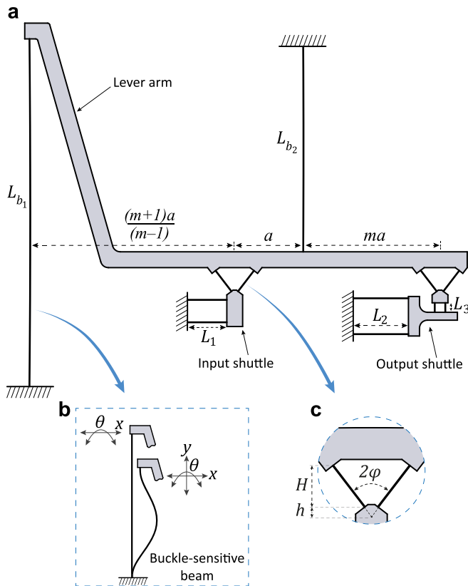
FIG. 1. (a) Schematic representation and geometric parameters of the frequency doubler transmission mechanism. (b) The buckle-sensitive beams are employed as a reconfigurable kinematic joint. (c) The geometric parameters of the double blade rotary pivot used in the design.
