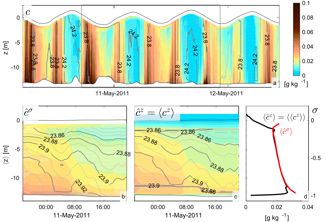
FIG. 5. As in Fig. 4, but for SPM concentration c .
