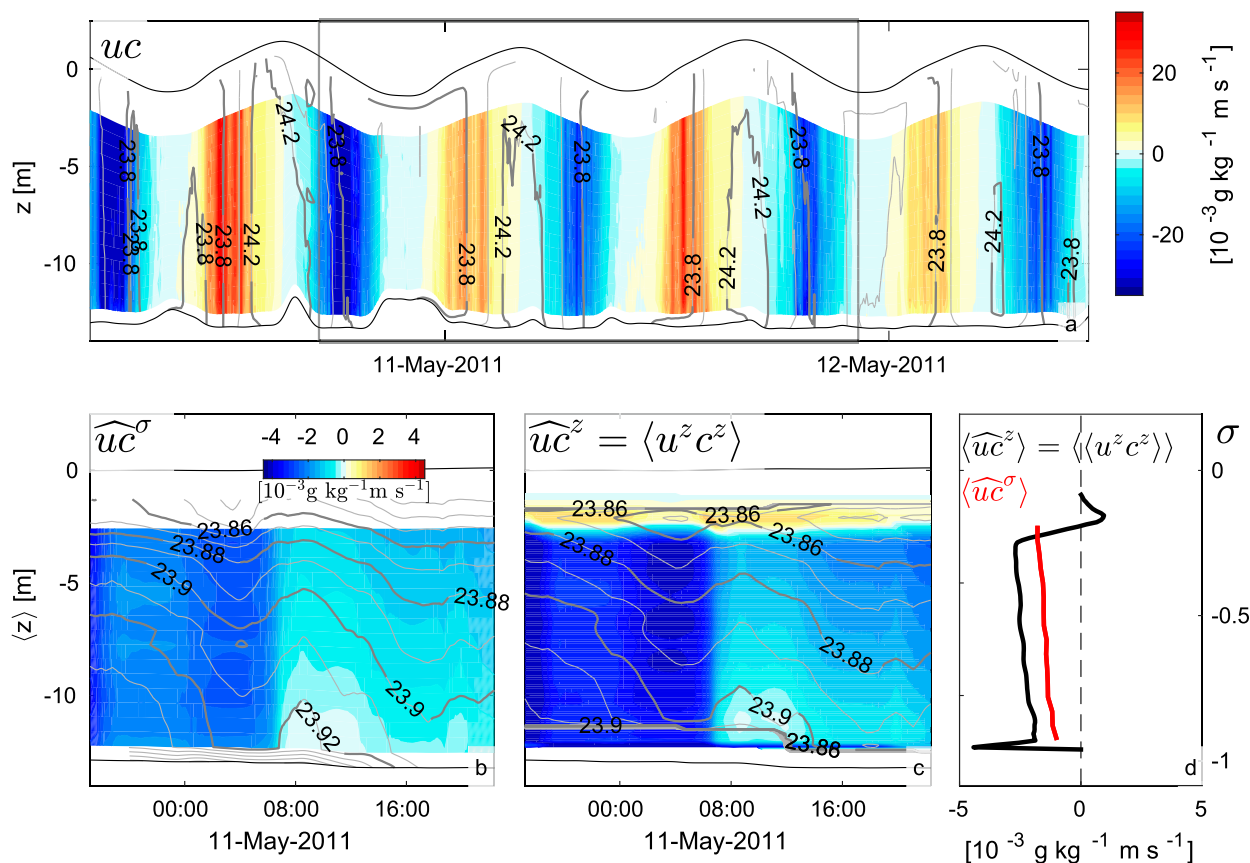
FIG. 6. As in Fig. 4, but for SPM flux uc .
