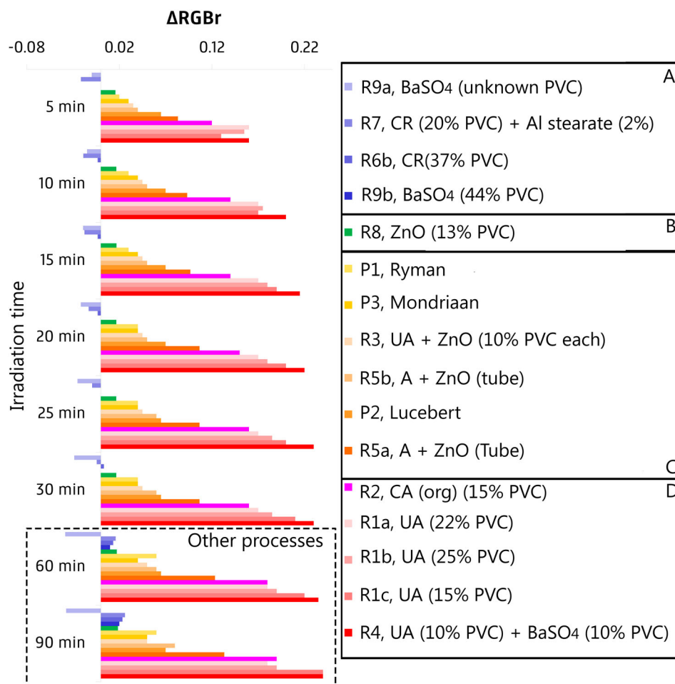
Figure 4. Complete dataset acquired via standard procedure ( \Delta RGB_r at all the different time intervals: 5, 10, 15, 20, 25, 30, 60, 90 min). If the sample was repeated, the average is shown. Four categories were discerned: A, stable; B, minor change; C, medium change; D, major change. At longer irradiation times (60, 90 min) other processes start to play a role (see text).
