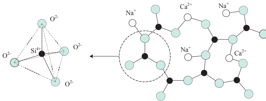
FIG. 2.28 Schematic representation of the structure of soda-lime silica glass based on (Louter 2011). Left: 3D schematic representation of a tetrahedral module built from one silicium and 4 oxide atoms. Right: 2D schematic representation of the irregular network of soda-lime silica glass.
