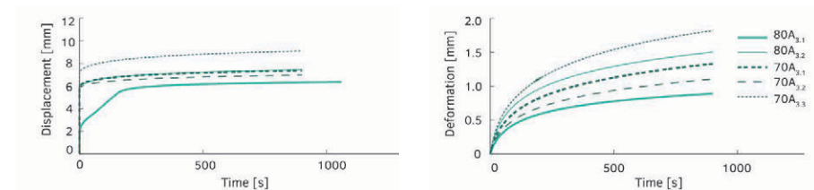
FIG. 8.15 Displacement in time graph of 70A_{3,x} and 80A_{3,x} specimens (left) and processed so that only the deformation in time under the static 40 kN load is shown (right)
