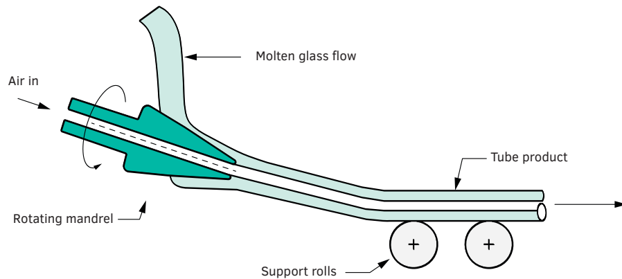
FIG. 2.5 Principle of the Danner process.
