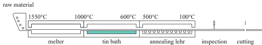
FIG. 2.1 Schematic illustration of the float production process by (Louter 2011) based on (Wörner et al. 2001).
