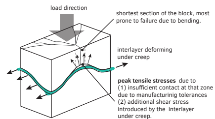
FIG. 8.10 Possible explanation of the cause of failure of the specimens interleaved with PMC770 (70A) and Task 16 (80A).
