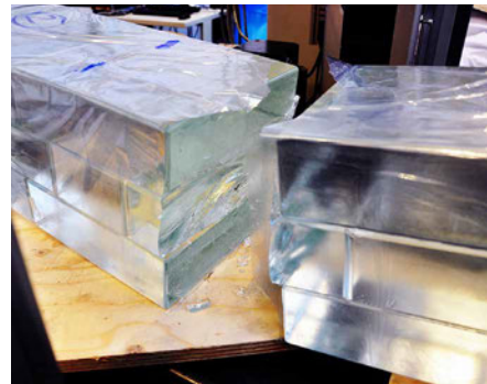
FIG. 5.26 Typical failure mode of specimens, a clear, vertical cut at the middle of the beam.
