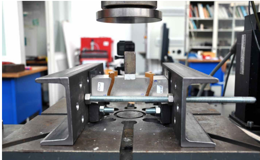
FIG. 8.26 Experimental set-up
