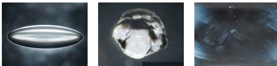
FIG. 2.30 Inclusion flaws in glass. From left to right: Bubbles, stones and cord. Source: (Molnár et al. 2012) and own image (right).
