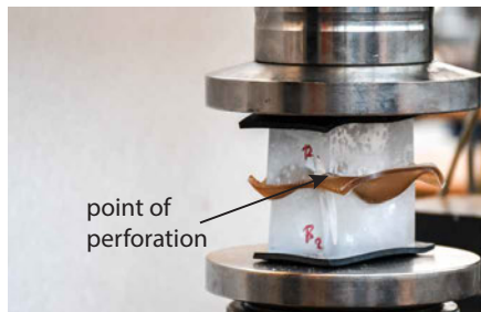
FIG. 8.12 Typical glass failure originating at the edge of the assembly caused by the perforation/tearing of the interlayer (specimen 60A 1 )
