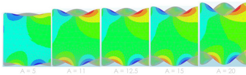
FIG. 8.41 Contour plots at failure load for various amplitude variations, demonstrating the stress redistribution of the given geometries. For the failure loads of each amplitude variation refer to Fig. 8.39. Source: (Jacobs 2017)
