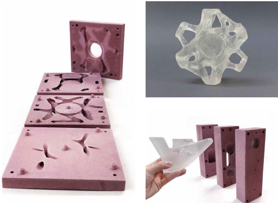
FIG. 2.27 3D-printed sand moulds produced by ExOne and the resulting cast glass components for a topologically optimized cast glass grid-shell node by (Damen 2019) (left and top right) and for a structurally optimized cast glass column by (Bhatia 2019) (bottom right).
