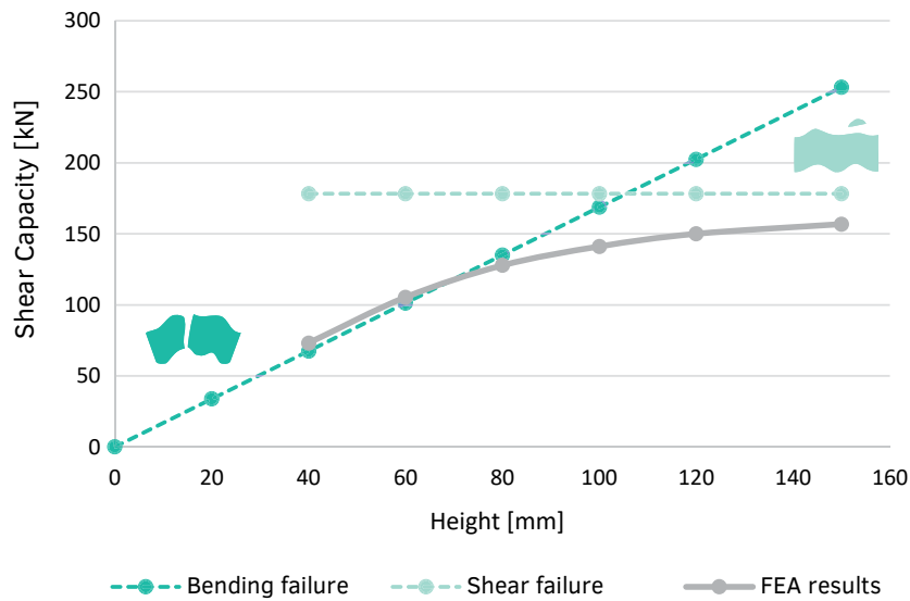
FIG. 8.42 The effect of the height on the shear capacity of the brick plotted together with the expectations from hand calculations. Source: (Jacobs 2017).
