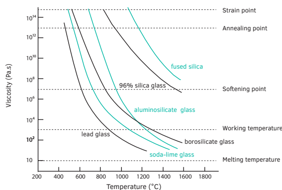
FIG. 2.18 Approximate viscosity versus temperature curves plot for the most characteristic glass families described in tables 2.1 and 2.2 based on (Shand, Armistead 1958).
