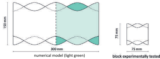
FIG. 8.33 Numerical model (Type B block) vs experimentally tested block (Type A).
