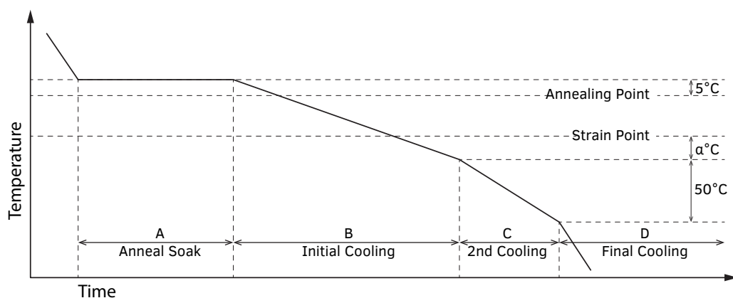
FIG. 2.20 Typical annealing scheme for commercial soda-lime glasses.
