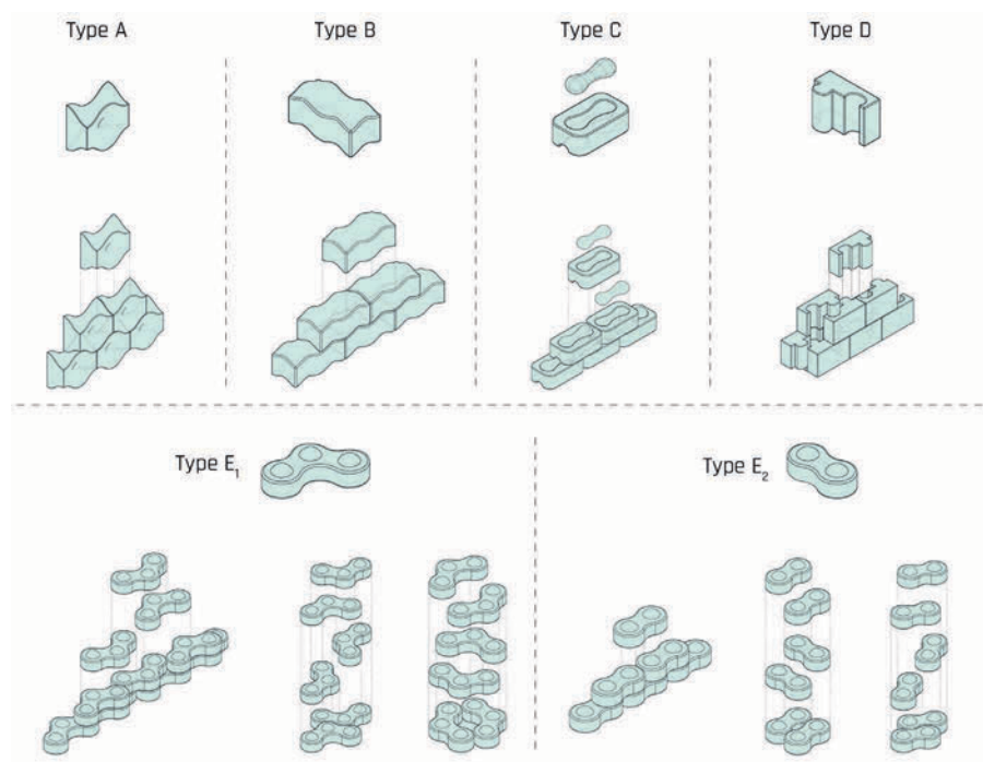
FIG. 7.6 Developed interlocking designs
