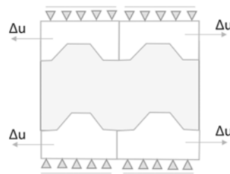
FIG. 8.36 (left) 2D Full scale principle of the model. Source:(Jacobs 2017).
