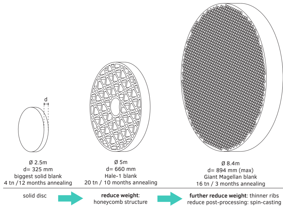
FIG. 3.8 Evolution of the cast mirror blanks in size and annealing times (Zirker 2005) due to smart geometry and improved manufacturing process.
