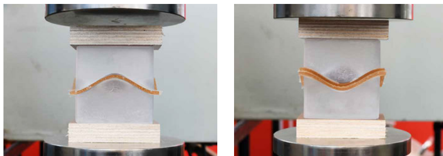
FIG. 8.8 Prototype with 70A interlayer of 3 mm thickness (left) and of 6 mm thickness (right).
