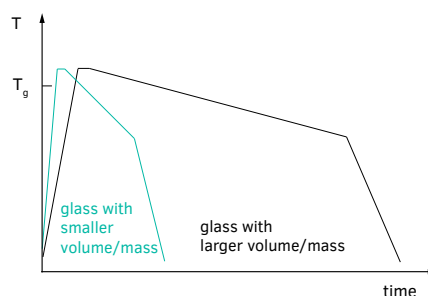
FIG. 2.19 Schematic representation of the annealing temperature as a function of time for glasses of different volume by (Schott AG 2004).
