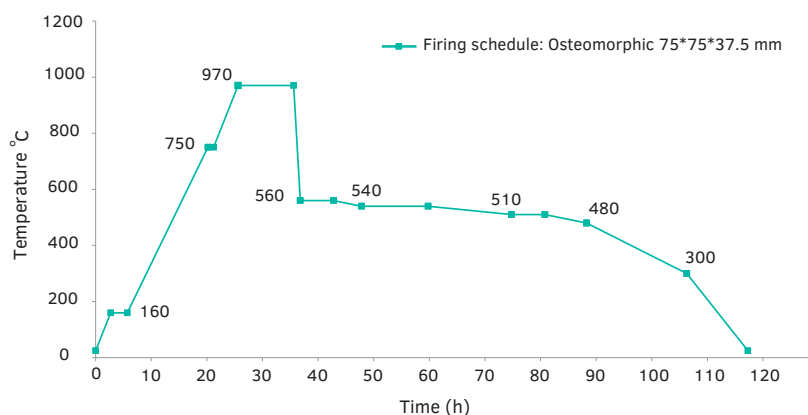
FIG. 8.1 Firing schedule followed for the kiln-casting and annealing of the osteomorphic blocks.
