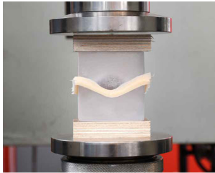
FIG. 8.21 A 6 mm thick 70A specimen before (left) and during (right) resting under 40 kN constant load
