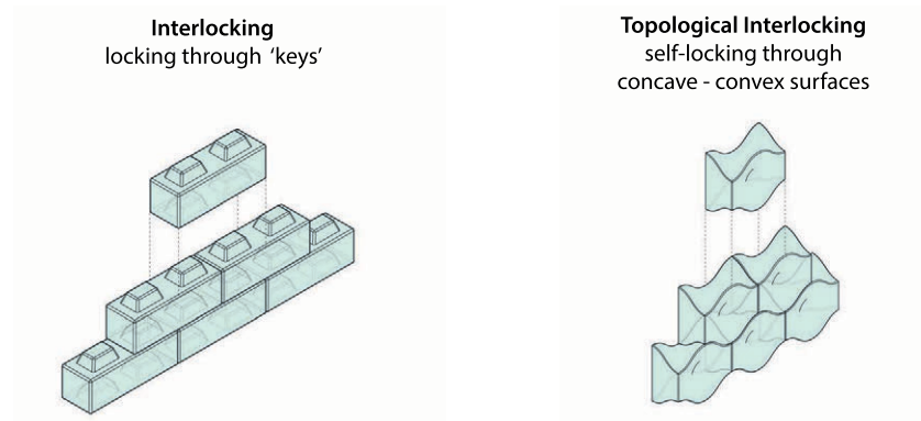
FIG. 7.1 Principle of interlocking and topological interlocking systems
