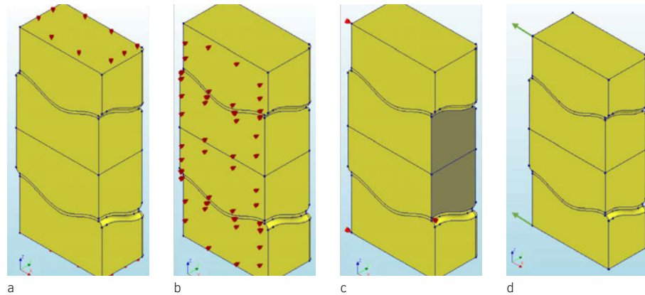
FIG. 8.38 Support conditions in a) Z-direction, b) Y-direction and c) X-direction. d) Tied vertices loaded with a prescribed deformation load. Source: (Jacobs 2017)
