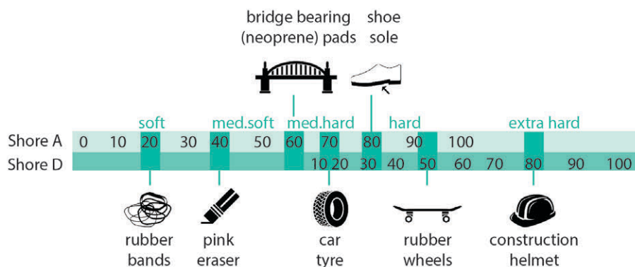
FIG. 7.16 Diagram of the shore hardness scales, including an indication of the shore hardness of common objects
