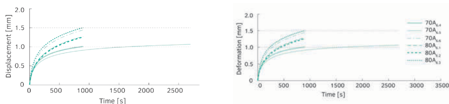
FIG. 8.17 Displacement in time ( u - t ) graph for the 70A and 80A 6 mm thick specimens tested to 40kN load for 900 s (left) and processed so that the deformation in time is shown only during the static 40 kN load (right).
