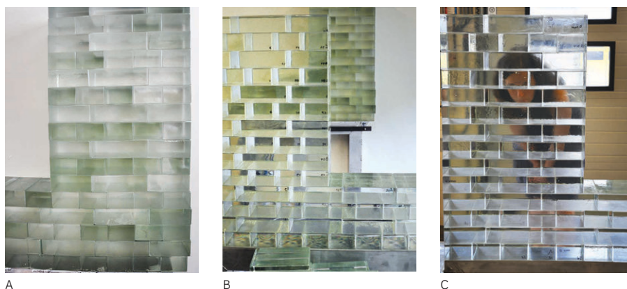
FIG. 5.7 Photographs of the three mock-ups. Mock-up A was made with higher tolerances. As a result there were significant offsets in both height and width, as well as open joints between blocks. Mock-up B was made with blocks of higher accuracy that prevented a substantial offset in height. Still, any unevenness up to \pm 0.5 mm in flatness resulted to cavities and bubbles in the bond area. In mock-up C all blocks meet the \pm 0.25 mm tolerance, resulting in an even spread of the adhesive and thus, in homogeneous bonding and satisfactory visual result without any cavities and bubbles of substantial dimensions.
