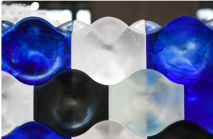
FIG. 7.21 Prototypes of the Type A osteomorphic topology made of recycled artware glass (blue), CRT screens (black), float glass (light blue) and optical lenses (clear) within the context of the Re 3 Glass project.
