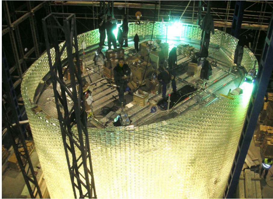
FIG. 4.12 Construction of the Atocha Memorial. Source: Bellapart, SAU.
