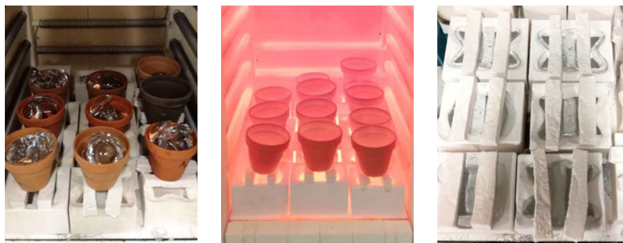
FIG. 8.2 From left to right: Arrangement of the glass-containing flowerpots above the crystal cast moulds and set-up of the kiln; View of the kiln at 970°C; Kiln-cast osteomorphic blocks prior to mould removal.
