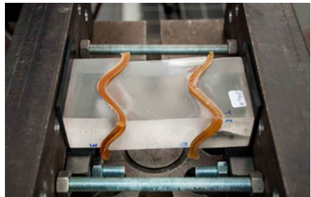
FIG. 8.31 Specimen out of blocks with 20 mm amplitude before testing (top left); at max. deformation (top right); and after failure (bottom left and right)
