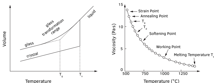
FIG. 2.17 Left: Schematic representation of the volume's dependence on temperature for a glass and a crystalline material. During the cooling process from a liquid to a solid, glasses do not convert to a crystalline state. Right: Typical curve for viscosity as a function of temperature for a soda-lime-silica melt (NIST Standard No. 710). Defined viscosity points are indicated on the figure. Source: (Shelby 2005).
