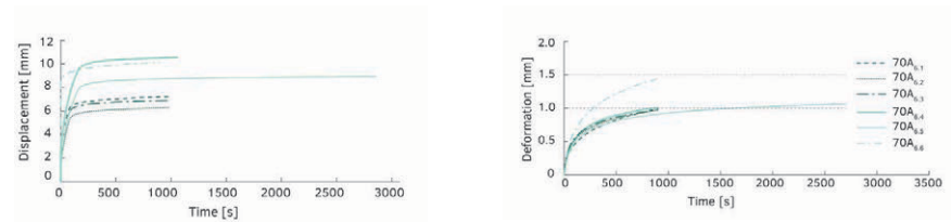
FIG. 8.20 Displacement in time ( u - t ) graph for 70A interlayer specimens, 6 mm thick tested under 20 kN ( 70A_{6.1} - 70A_{6.3} ) and 40 kN ( 70A_{6.4} - 70A_{6.6} ) load for 900s (left) and processed graph so that the deformation in time is shown only during the set constant loads (right).
