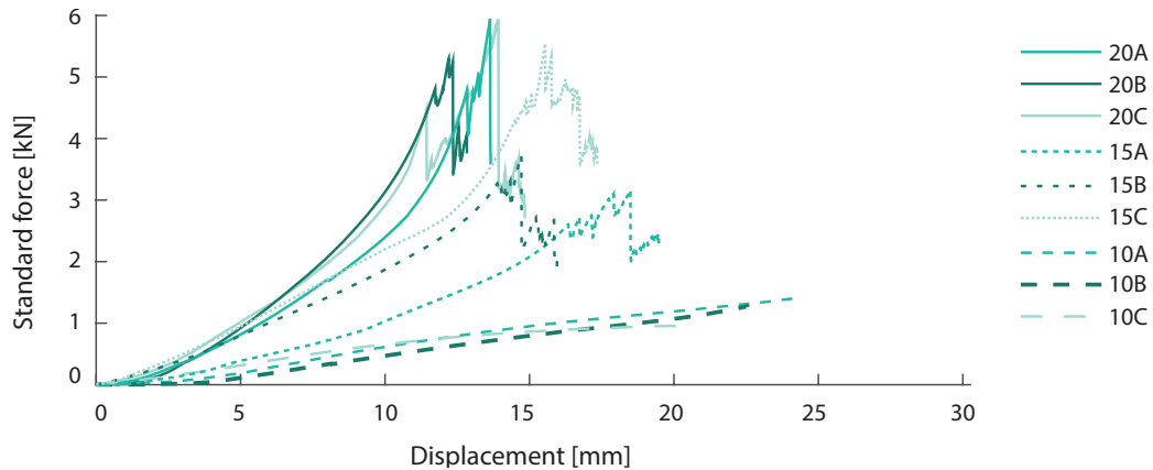
FIG. 8.27 Displacement - Standard Force diagram for all specimens
