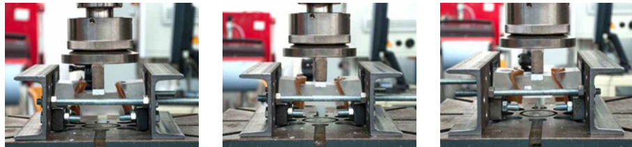
FIG. 8.28 Maximum deformation prior to failure of assemblies with blocks of 10 mm (left), 15 mm (center) and 20 mm (right) amplitude. The tests with blocks of 10 mm amplitude were aborted once the assembly reached an apparent deformation of 25 mm.
