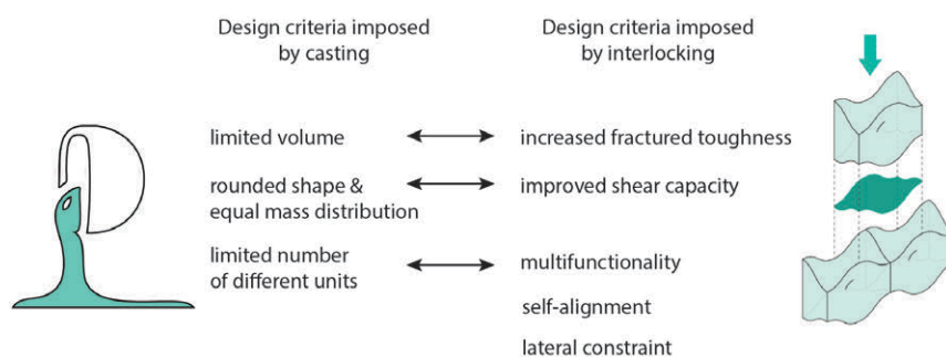
FIG. 7.5 Overview of the established design criteria. The double arrows indicate the alignment between the two different sets of criteria, due to casting and due to interlocking
