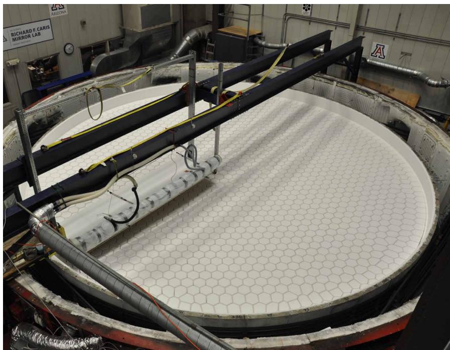
FIG. 3.3 Disposable mould for the blanks of the Giant Magellan Telescope built within the bottom part of the rotating kiln at the Steward Observatory in Arizona.
