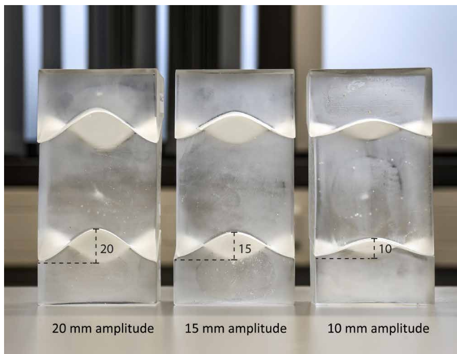
FIG. 8.24 Assemblies (without the use of an interlayer) of blocks with the different examined amplitudes.
