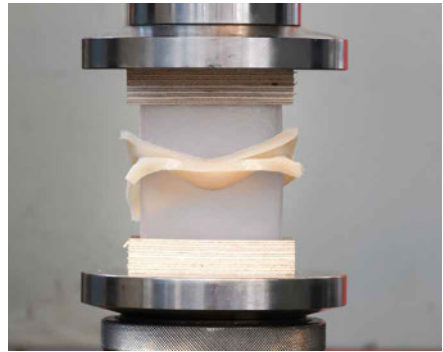
FIG. 8.21 A 6 mm thick 70A specimen before (left) and during (right) resting under 40 kN constant load
