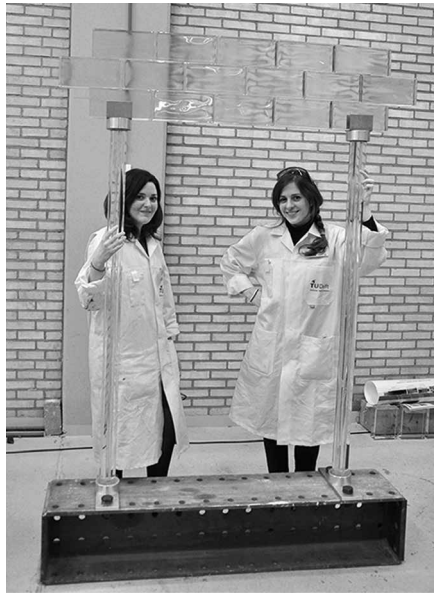
FIG. 2.7 Left: 1.5 m long bundled glass columns at TU Delft Glass Lab . Top right: Extrusion profiles made by SCHOTT AG . Bottom right: A bundled glass column made of adhesively bonded extruded profiles developed by (Oikonomopoulou et al. 2017b).
