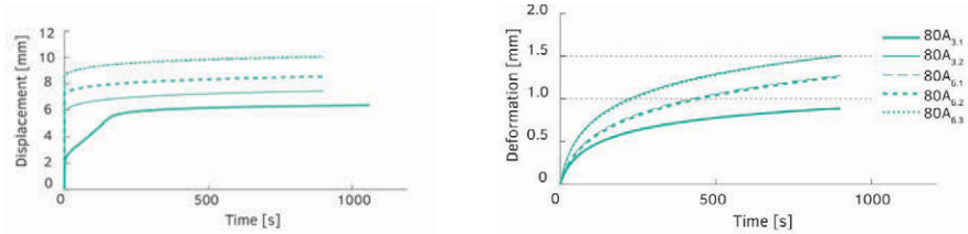
FIG. 8.18 Displacement in time ( u - t ) graph for the 80A interlayer specimens of 3 mm and 6 mm thickness tested under 40 kN load for 900s (left) and processed graph so that the deformation in time is shown only during the set 40kN constant load (right).
