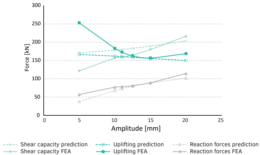
FIG. 8.40 Influence of amplitude on shear capacity, uplifting force (parallel to interlock curvature) and reaction forces. The prediction lines are based on hand calculations described in (Jacobs 2017).
