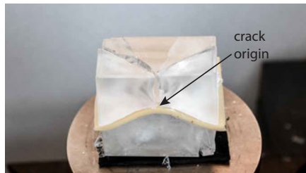
FIG. 8.9 Typical Y breaking pattern originating at the shortest section of the block (specimen 80A 1 )
