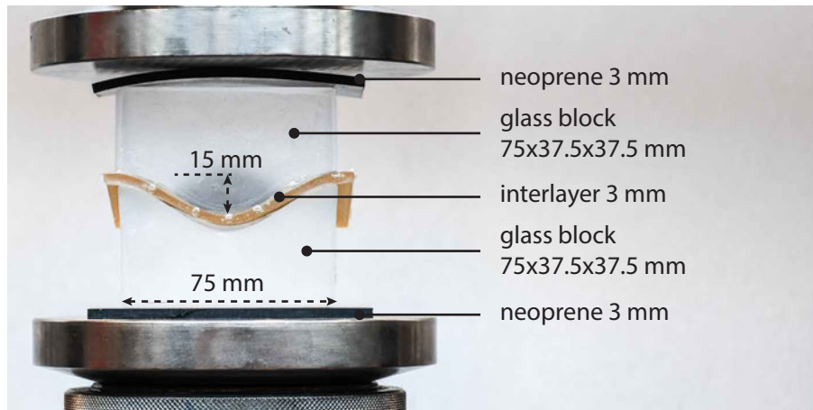
FIG. 8.5 Experimental set-up
