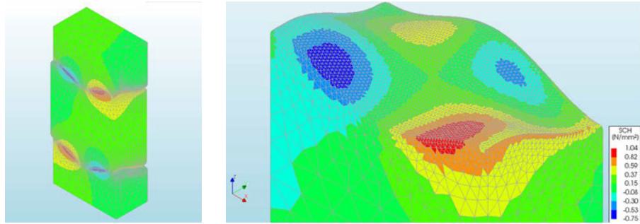
FIG. 8.35 Left: Numerical set up and results for Christensen's failure criterion value of one ( SCH=1 ) of the tested variants. Right: Christensen's output ( SCH=1 ) of middle brick (amplitude 10 mm). Shear capacity at failure is approximately 155 kN. Source:(Jacobs 2017).
