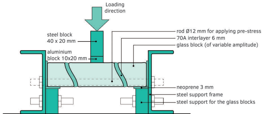
FIG. 8.25 Illustration of the experimental set-up.
