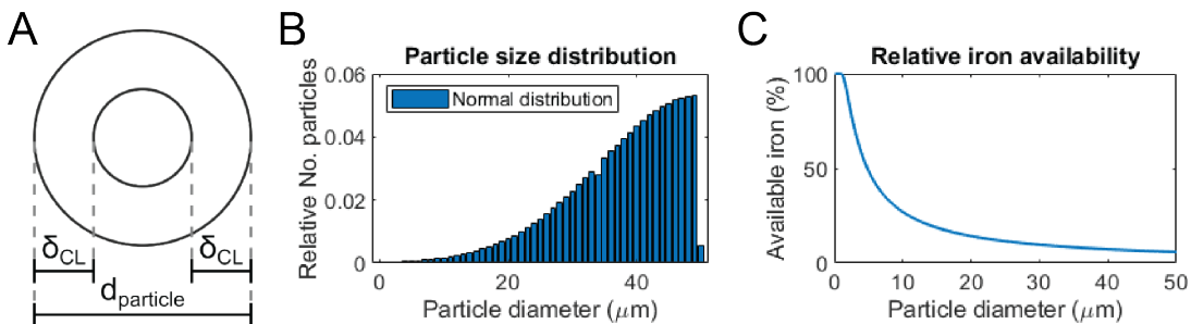
Fig. 8.4 (A) Visualization of the contact layer model. (B) Expected particle size distribution grouped in bars of 1 \mu m . (C) Iron availability for each particle diameter, decreasing with particle size.
