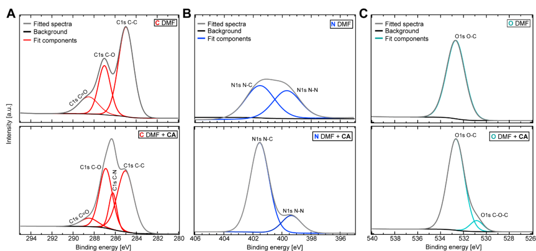
Fig. 4.5 X-ray photoelectron spectroscopy (XPS) analysis of CA-functionalized of GO in DMF. (A) Carbon, (B) nitrogen, and (C) oxygen XPS spectra before (top panels) and after (bottom panels) addition of CA. A carbon-nitrogen binding exhibited the best fit for the XPS spectrum with CA treatment (bottom panels), reflecting a 2-fold increase in peak intensity. Grey lines represent deconvoluted multi-peak fittings.
